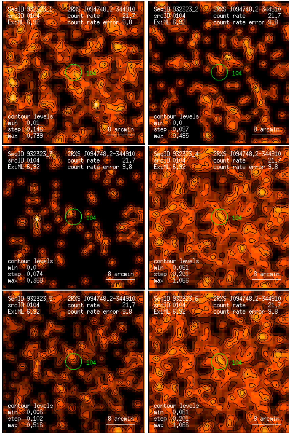
Figure 104: RASS 932323: detection 0104: band rate images, Gaussian filter: (1) PSPC channels 11 – 41, (2) 52 – 90, (3) 91 – 201, (4) 11 – 235, (5) 52 – 201, (6) 11 – 201. Broad band rates in counts/ks. Band rate contour levels in counts/ks/arcmin 2 .
