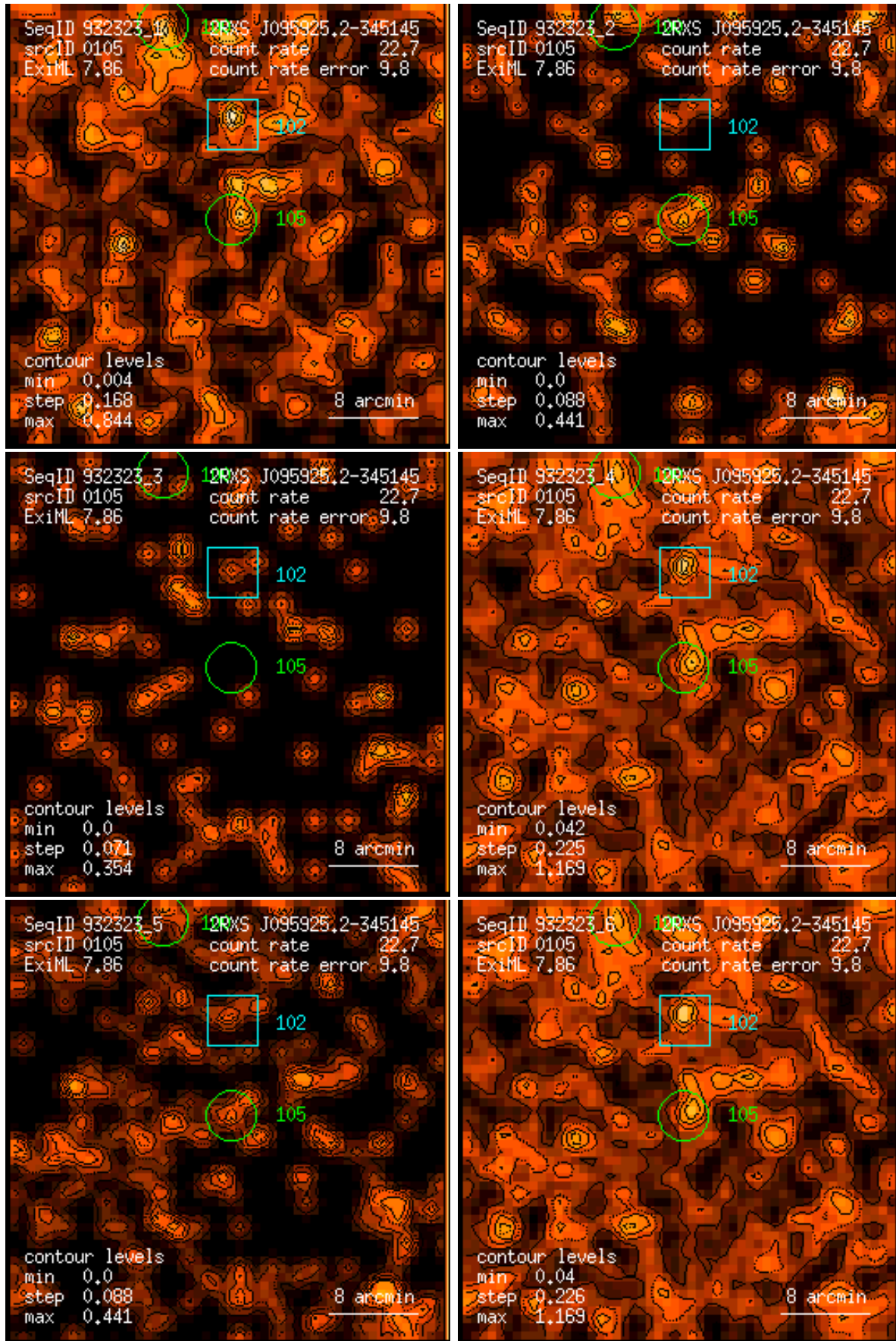
Figure 105: RASS 932323: detection 0105: band rate images, Gaussian filter: (1) PSPC channels 11 – 41, (2) 52 – 90, (3) 91 – 201, (4) 11 – 235, (5) 52 – 201, (6) 11 – 201. Broad band rates in counts/ks. Band rate contour levels in counts/ks/arcmin 2 .
