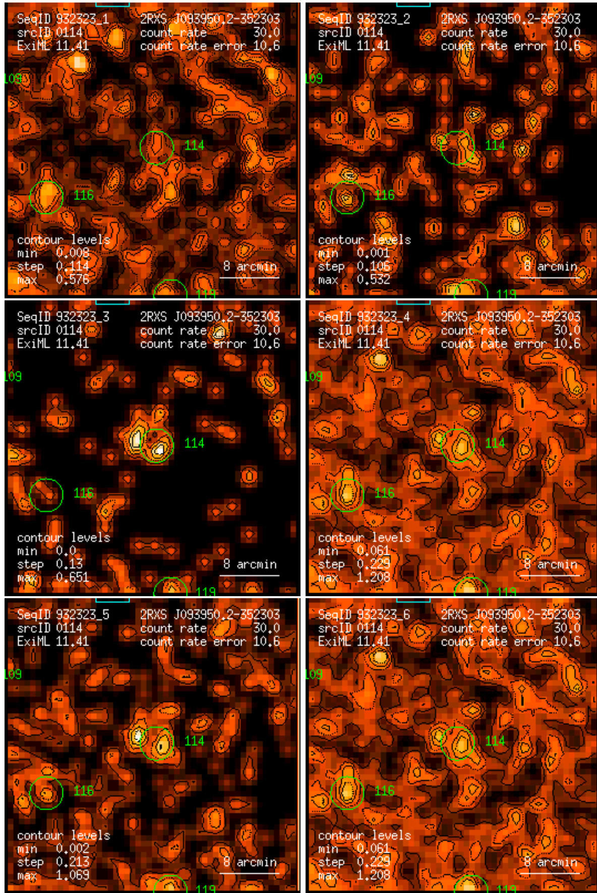
Figure 114: RASS 932323: detection 0114: band rate images, Gaussian filter: (1) PSPC channels 11 – 41, (2) 52 – 90, (3) 91 – 201, (4) 11 – 235, (5) 52 – 201, (6) 11 – 201. Broad band rates in counts/ks. Band rate contour levels in counts/ks/arcmin 2 .
