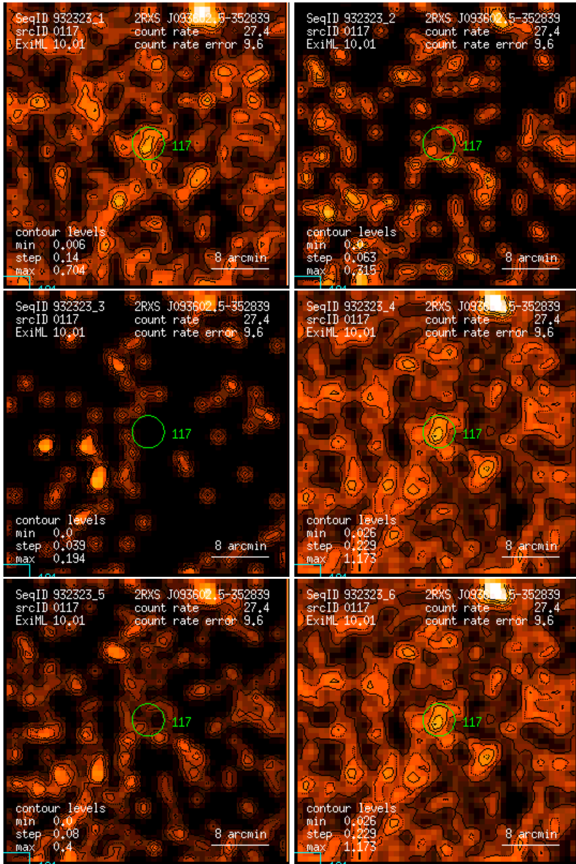
Figure 117: RASS 932323: detection 0117: band rate images, Gaussian filter: (1) PSPC channels 11 – 41, (2) 52 – 90, (3) 91 – 201, (4) 11 – 235, (5) 52 – 201, (6) 11 – 201. Broad band rates in counts/ks. Band rate contour levels in counts/ks/arcmin 2 .
