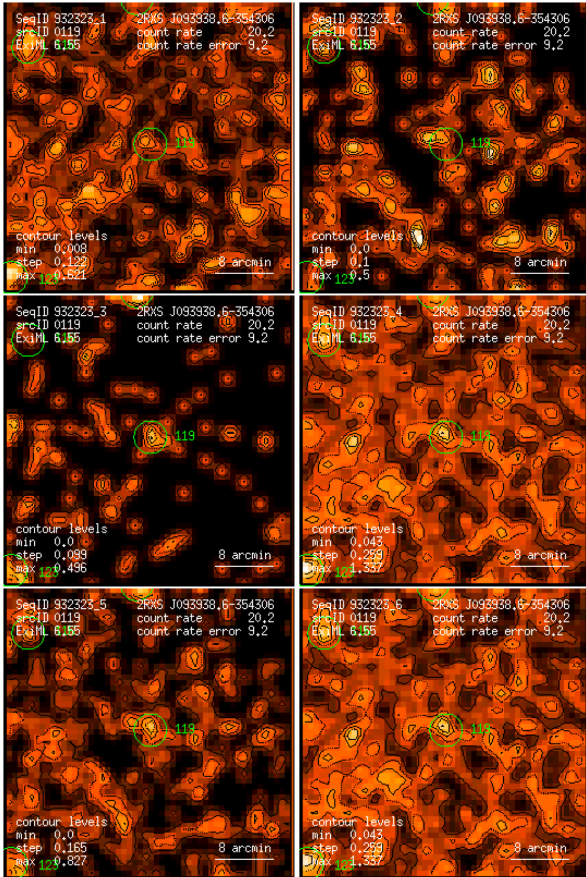
Figure 119: RASS 932323: detection 0119: band rate images, Gaussian filter: (1) PSPC channels 11 – 41, (2) 52 – 90, (3) 91 – 201, (4) 11 – 235, (5) 52 – 201, (6) 11 – 201. Broad band rates in counts/ks. Band rate contour levels in counts/ks/arcmin 2 .
