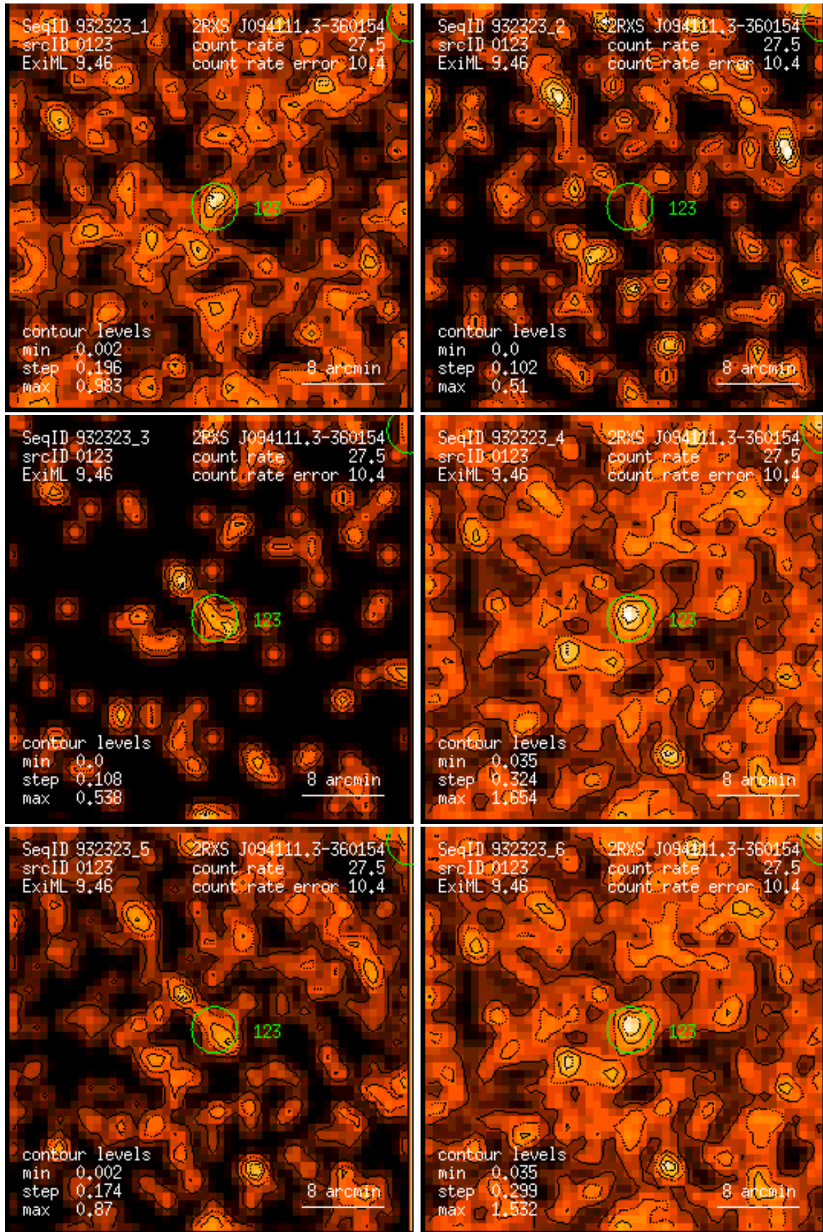
Figure 123: RASS 932323: detection 0123: band rate images, Gaussian filter: (1) PSPC channels 11 – 41, (2) 52 – 90, (3) 91 – 201, (4) 11 – 235, (5) 52 – 201, (6) 11 – 201. Broad band rates in counts/ks. Band rate contour levels in counts/ks/arcmin 2 .
