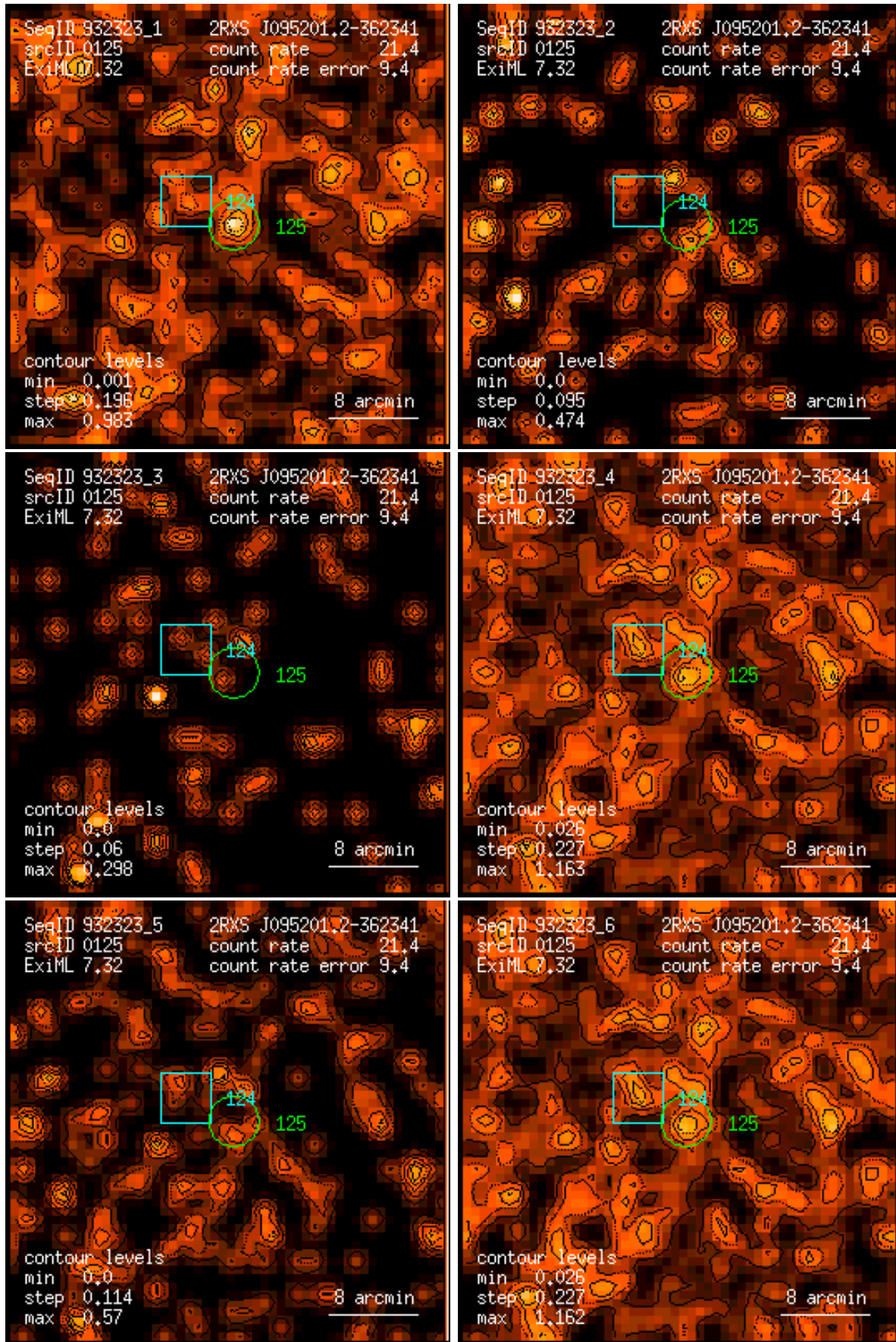
Figure 125: RASS 932323: detection 0125: band rate images, Gaussian filter: (1) PSPC channels 11 – 41, (2) 52 – 90, (3) 91 – 201, (4) 11 – 235, (5) 52 – 201, (6) 11 – 201. Broad band rates in counts/ks. Band rate contour levels in counts/ks/arcmin 2 .
