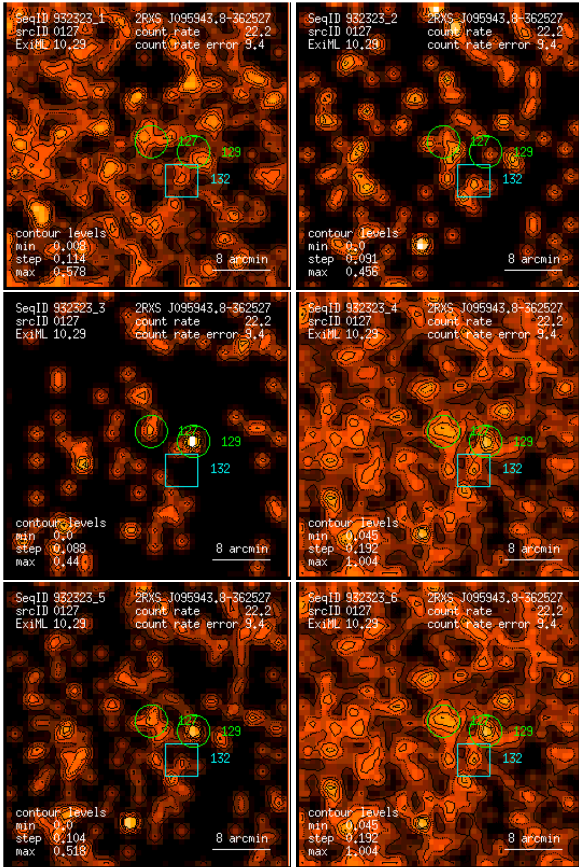
Figure 127: RASS 932323: detection 0127: band rate images, Gaussian filter: (1) PSPC channels 11 – 41, (2) 52 – 90, (3) 91 – 201, (4) 11 – 235, (5) 52 – 201, (6) 11 – 201. Broad band rates in counts/ks. Band rate contour levels in counts/ks/arcmin 2 .
