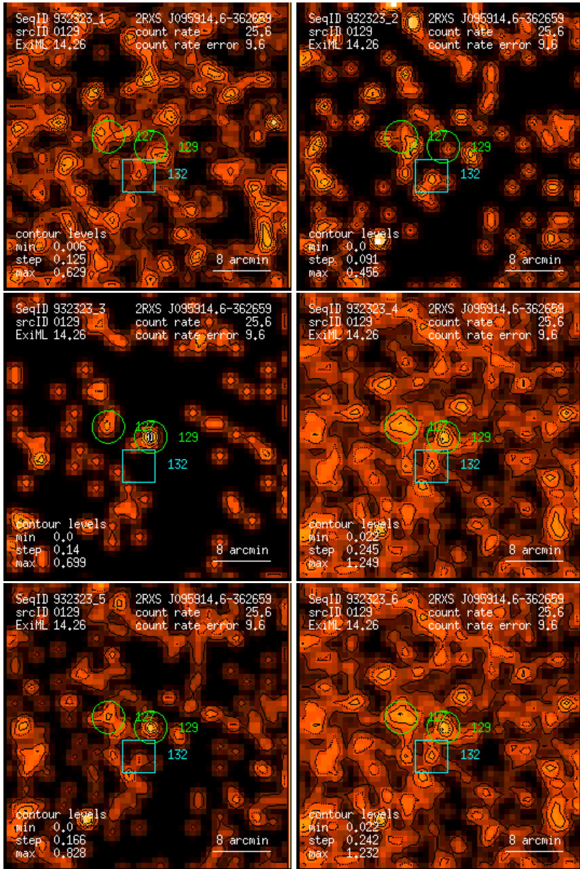
Figure 129: RASS 932323: detection 0129: band rate images, Gaussian filter: (1) PSPC channels 11 – 41, (2) 52 – 90, (3) 91 – 201, (4) 11 – 235, (5) 52 – 201, (6) 11 – 201. Broad band rates in counts/ks. Band rate contour levels in counts/ks/arcmin 2 .
