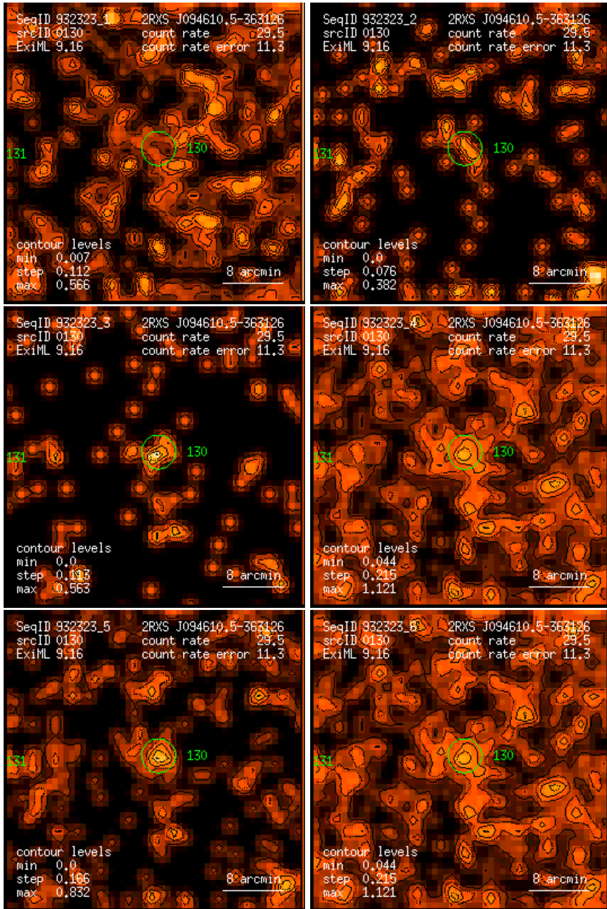
Figure 130: RASS 932323: detection 0130: band rate images, Gaussian filter: (1) PSPC channels 11 – 41, (2) 52 – 90, (3) 91 – 201, (4) 11 – 235, (5) 52 – 201, (6) 11 – 201. Broad band rates in counts/ks. Band rate contour levels in counts/ks/arcmin 2 .
