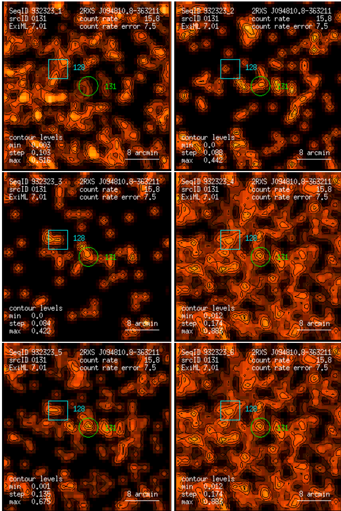
Figure 131: RASS 932323: detection 0131: band rate images, Gaussian filter: (1) PSPC channels 11 – 41, (2) 52 – 90, (3) 91 – 201, (4) 11 – 235, (5) 52 – 201, (6) 11 – 201. Broad band rates in counts/ks. Band rate contour levels in counts/ks/arcmin 2 .
