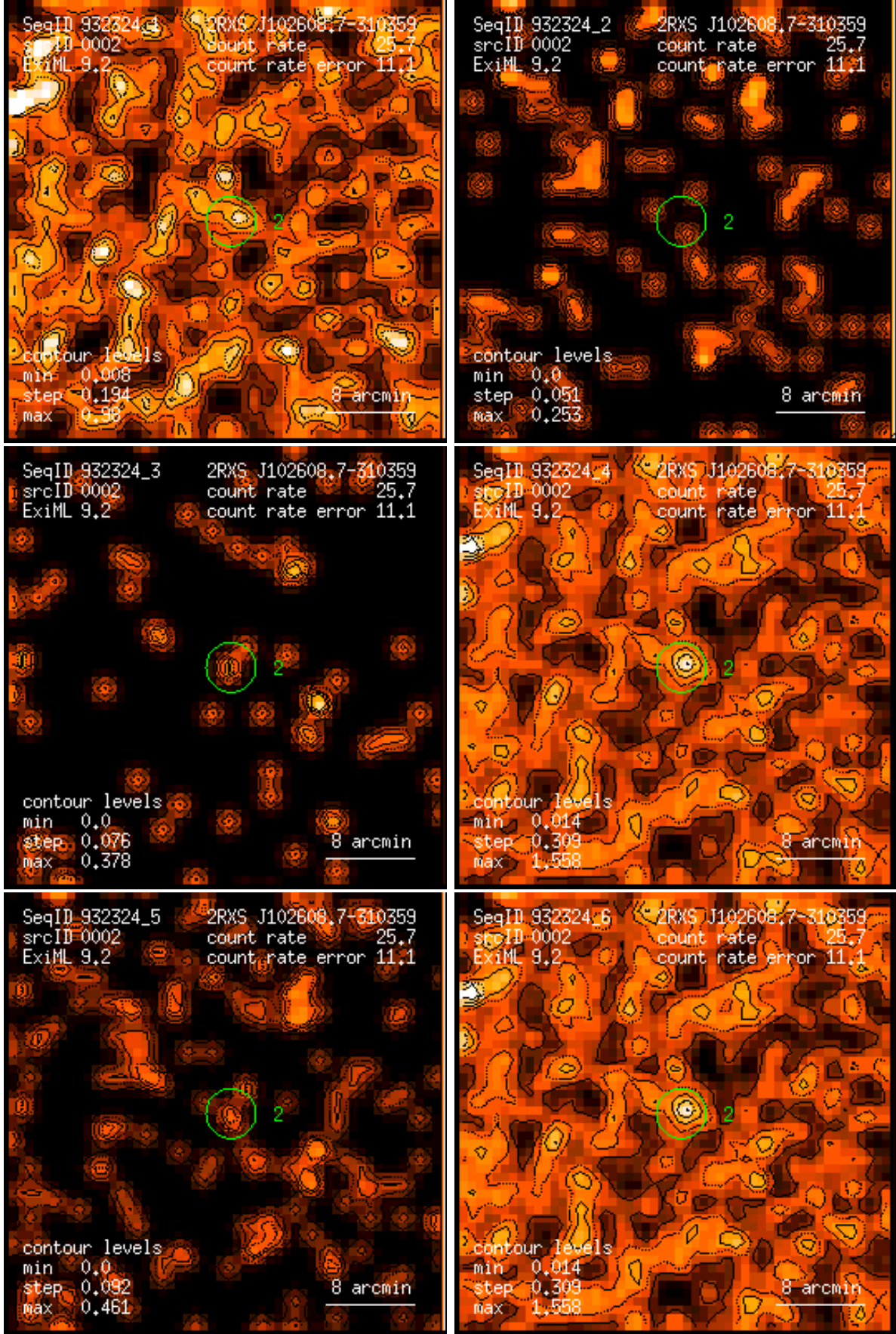
Figure 2: RASS 932324: detection 0002: band rate images, Gaussian filter: (1) PSPC channels 11 – 41, (2) 52 – 90, (3) 91 – 201, (4) 11 – 235, (5) 52 – 201, (6) 11 – 201. Broad band rates in counts/ks. Band rate contour levels in counts/ks/arcmin 2 .
