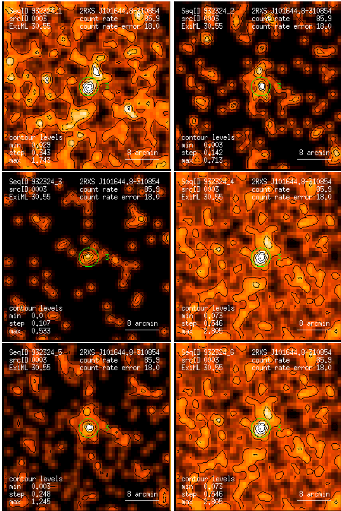
Figure 3: RASS 932324: detection 0003: band rate images, Gaussian filter: (1) PSPC channels 11 – 41, (2) 52 – 90, (3) 91 – 201, (4) 11 – 235, (5) 52 – 201, (6) 11 – 201. Broad band rates in counts/ks. Band rate contour levels in counts/ks/arcmin 2 .
