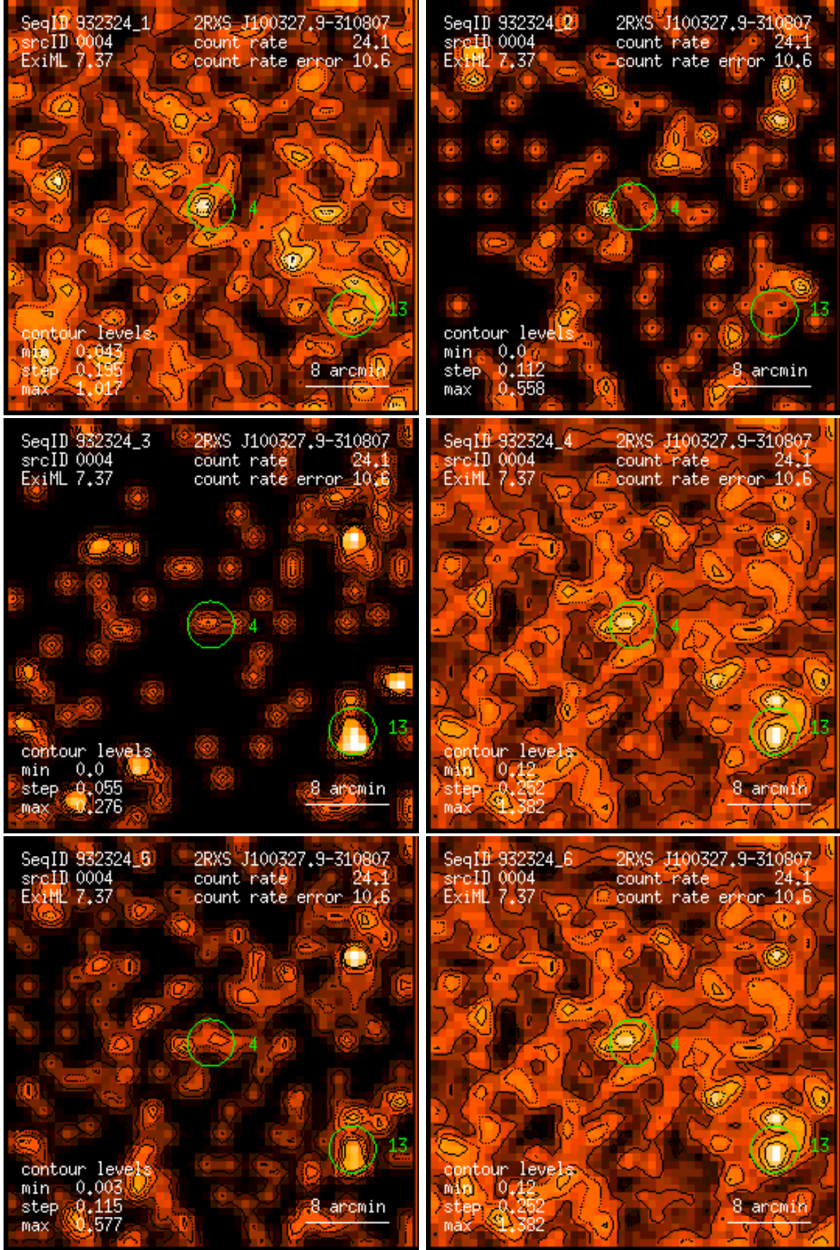
Figure 4: RASS 932324: detection 0004: band rate images, Gaussian filter: (1) PSPC channels 11 – 41, (2) 52 – 90, (3) 91 – 201, (4) 11 – 235, (5) 52 – 201, (6) 11 – 201. Broad band rates in counts/ks. Band rate contour levels in counts/ks/arcmin 2 .
