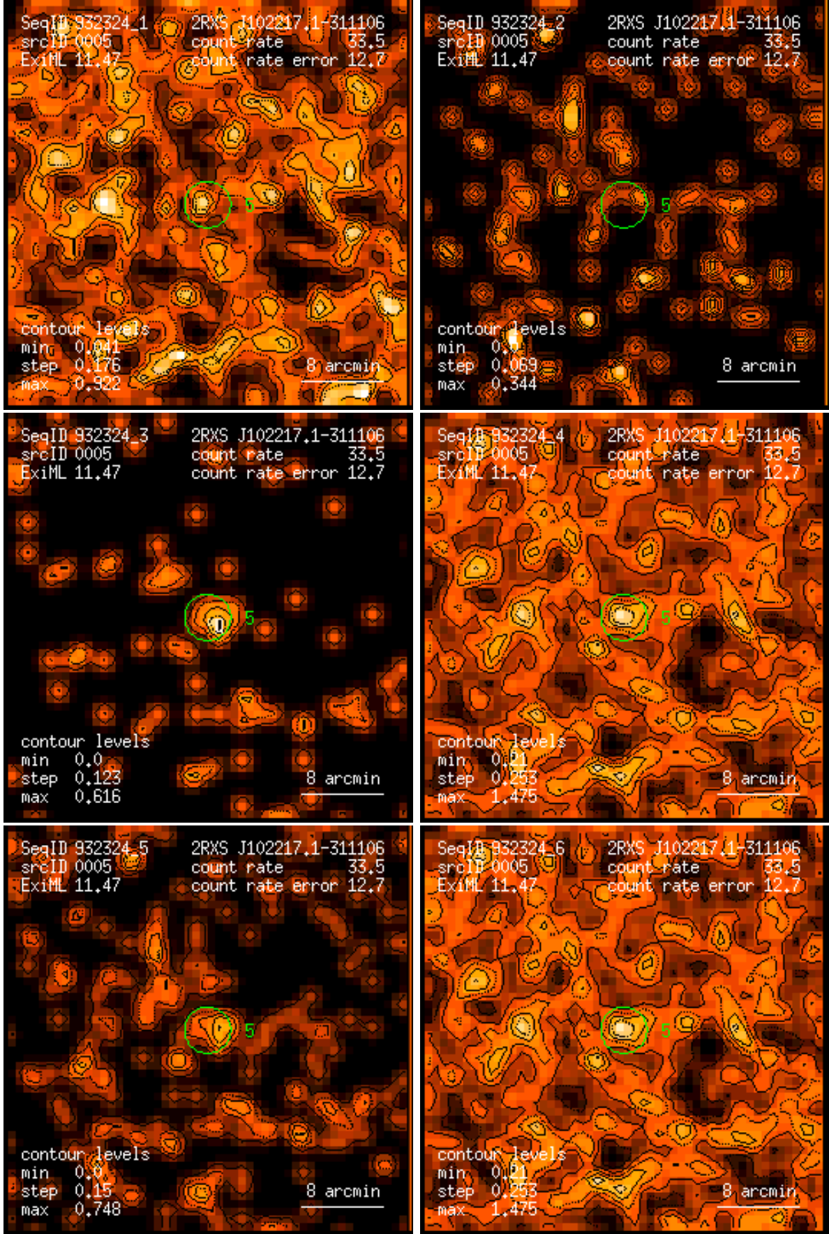
Figure 5: RASS 932324: detection 0005: band rate images, Gaussian filter: (1) PSPC channels 11 – 41, (2) 52 – 90, (3) 91 – 201, (4) 11 – 235, (5) 52 – 201, (6) 11 – 201. Broad band rates in counts/ks. Band rate contour levels in counts/ks/arcmin 2 .
