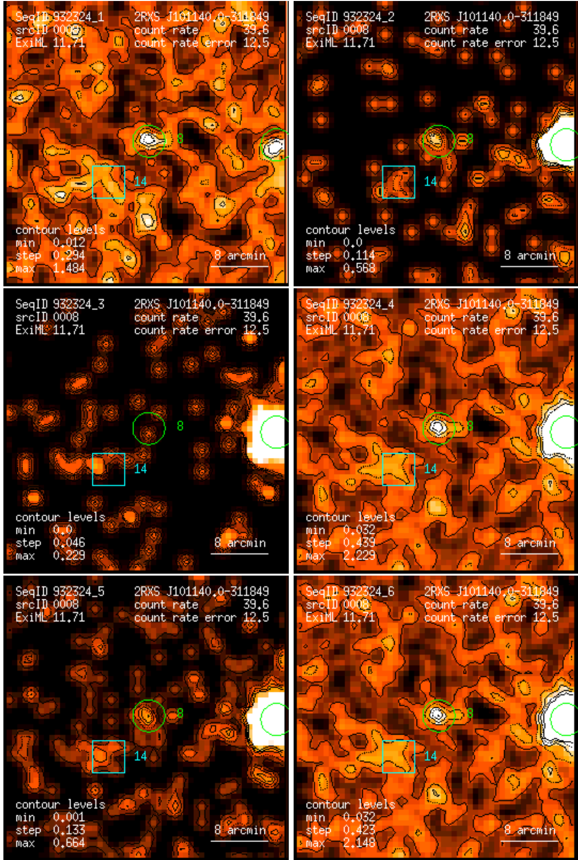
Figure 8: RASS 932324: detection 0008: band rate images, Gaussian filter: (1) PSPC channels 11 – 41, (2) 52 – 90, (3) 91 – 201, (4) 11 – 235, (5) 52 – 201, (6) 11 – 201. Broad band rates in counts/ks. Band rate contour levels in counts/ks/arcmin 2 .
