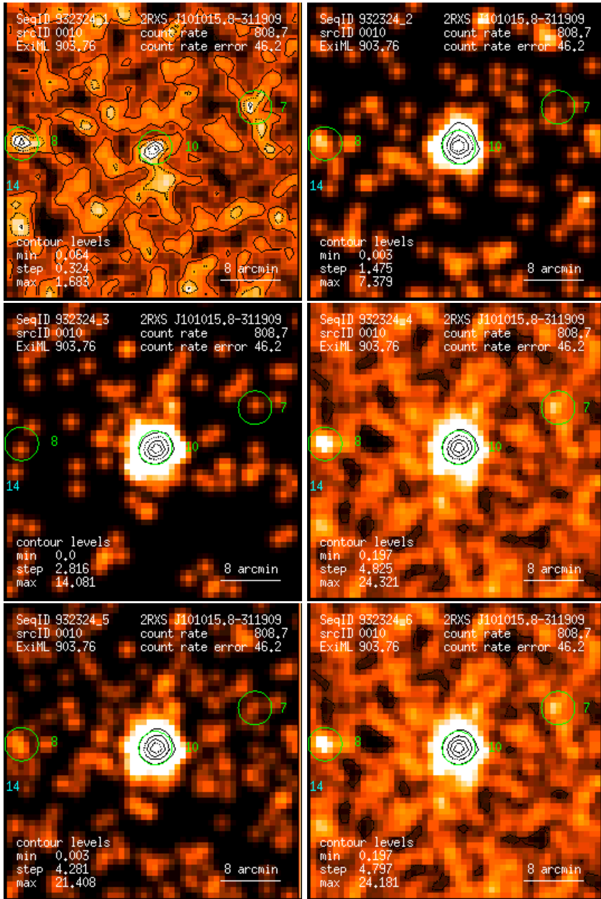
Figure 10: RASS 932324: detection 0010: band rate images, Gaussian filter: (1) PSPC channels 11 – 41, (2) 52 – 90, (3) 91 – 201, (4) 11 – 235, (5) 52 – 201, (6) 11 – 201. Broad band rates in counts/ks. Band rate contour levels in counts/ks/arcmin 2 .
