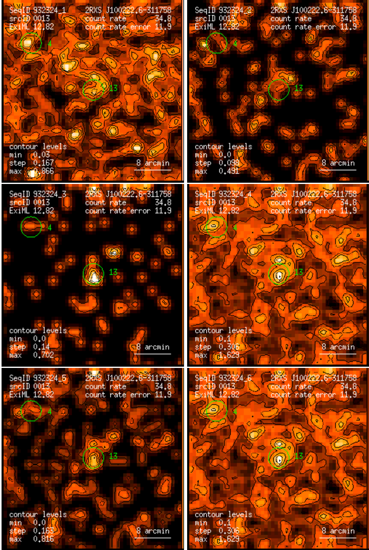
Figure 13: RASS 932324: detection 0013: band rate images, Gaussian filter: (1) PSPC channels 11 – 41, (2) 52 – 90, (3) 91 – 201, (4) 11 – 235, (5) 52 – 201, (6) 11 – 201. Broad band rates in counts/ks. Band rate contour levels in counts/ks/arcmin 2 .
