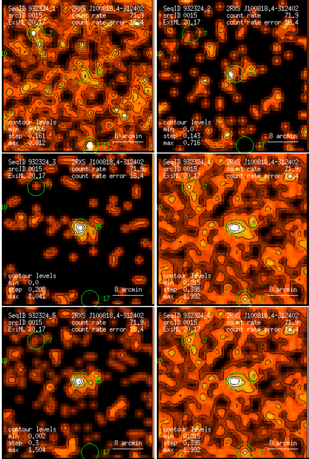
Figure 15: RASS 932324: detection 0015: band rate images, Gaussian filter: (1) PSPC channels 11 – 41, (2) 52 – 90, (3) 91 – 201, (4) 11 – 235, (5) 52 – 201, (6) 11 – 201. Broad band rates in counts/ks. Band rate contour levels in counts/ks/arcmin 2 .
