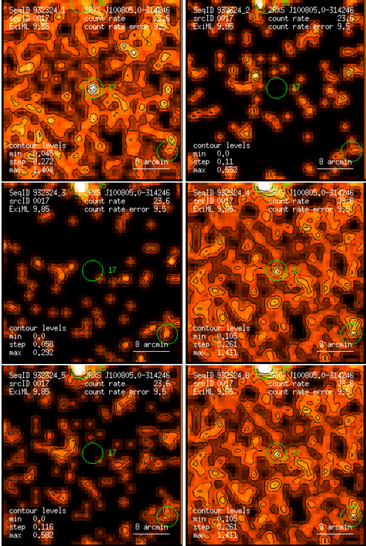
Figure 17: RASS 932324: detection 0017: band rate images, Gaussian filter: (1) PSPC channels 11 – 41, (2) 52 – 90, (3) 91 – 201, (4) 11 – 235, (5) 52 – 201, (6) 11 – 201. Broad band rates in counts/ks. Band rate contour levels in counts/ks/arcmin 2 .
