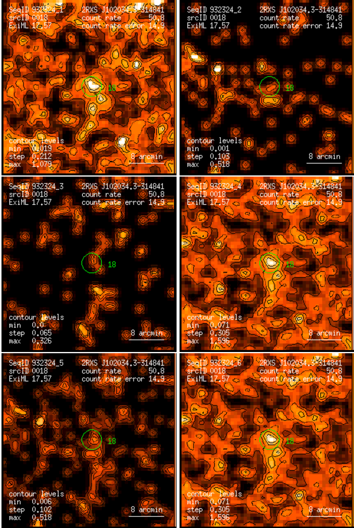
Figure 18: RASS 932324: detection 0018: band rate images, Gaussian filter: (1) PSPC channels 11 – 41, (2) 52 – 90, (3) 91 – 201, (4) 11 – 235, (5) 52 – 201, (6) 11 – 201. Broad band rates in counts/ks. Band rate contour levels in counts/ks/arcmin 2 .
