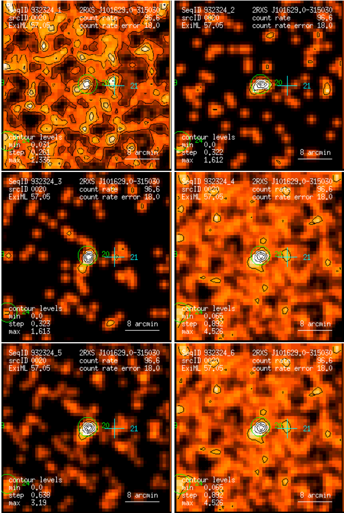
Figure 20: RASS 932324: detection 0020: band rate images, Gaussian filter: (1) PSPC channels 11 – 41, (2) 52 – 90, (3) 91 – 201, (4) 11 – 235, (5) 52 – 201, (6) 11 – 201. Broad band rates in counts/ks. Band rate contour levels in counts/ks/arcmin 2 .
