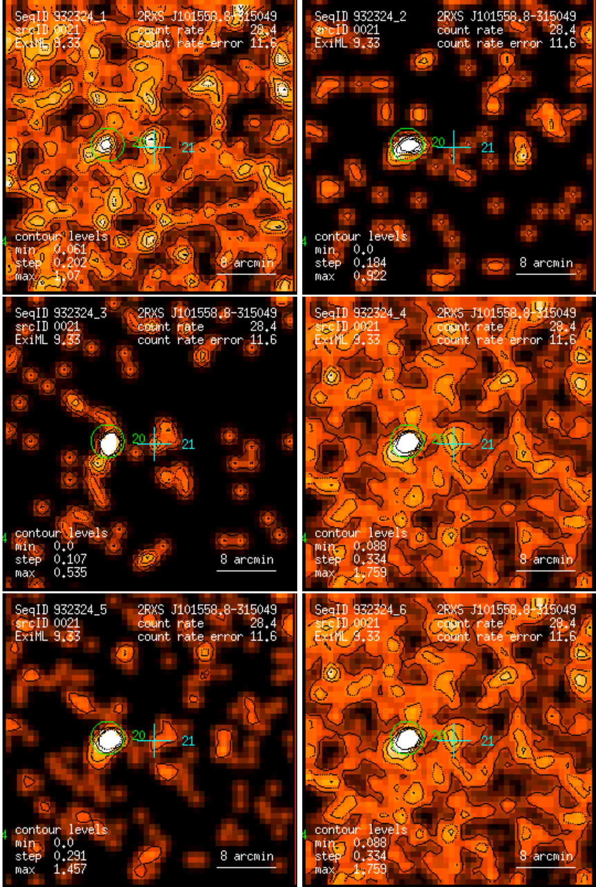
Figure 21: RASS 932324: detection 0021: band rate images, Gaussian filter: (1) PSPC channels 11 – 41, (2) 52 – 90, (3) 91 – 201, (4) 11 – 235, (5) 52 – 201, (6) 11 – 201. Broad band rates in counts/ks. Band rate contour levels in counts/ks/arcmin 2 .
