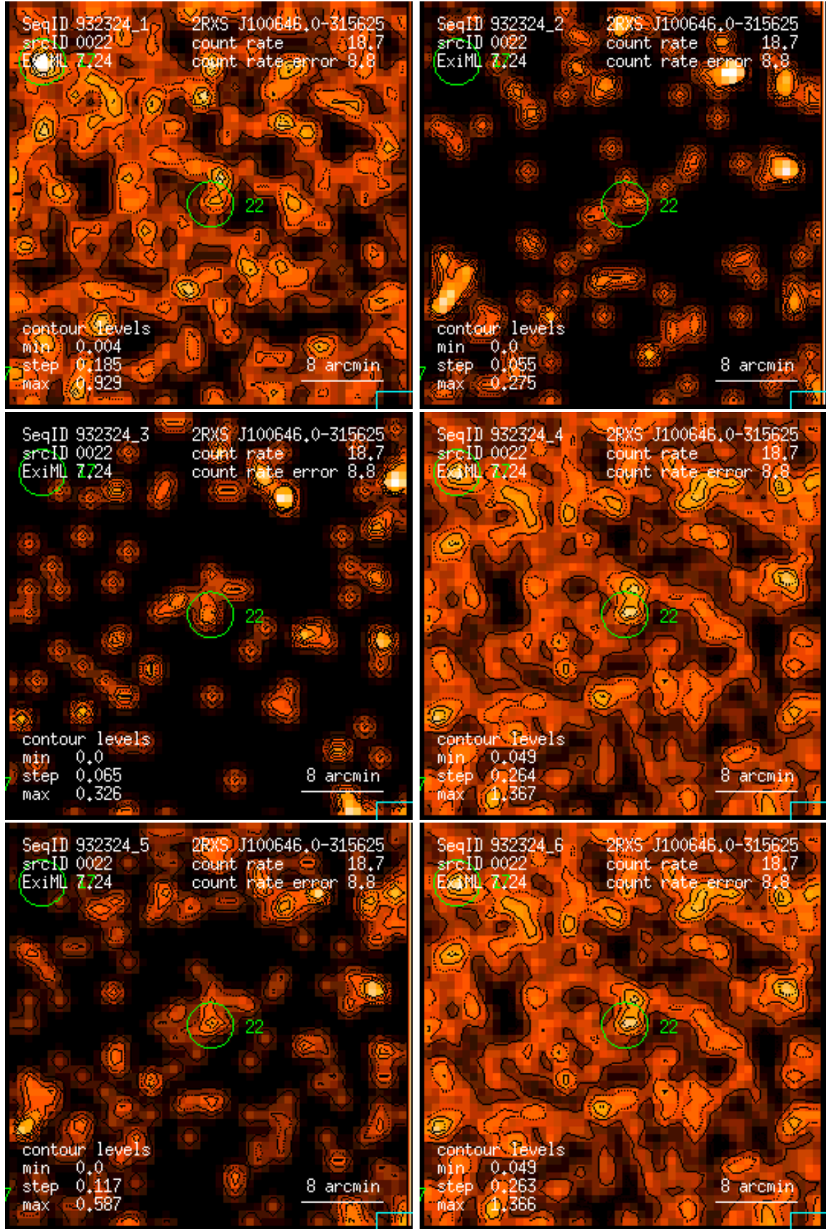
Figure 22: RASS 932324: detection 0022: band rate images, Gaussian filter: (1) PSPC channels 11 – 41, (2) 52 – 90, (3) 91 – 201, (4) 11 – 235, (5) 52 – 201, (6) 11 – 201. Broad band rates in counts/ks. Band rate contour levels in counts/ks/arcmin 2 .
