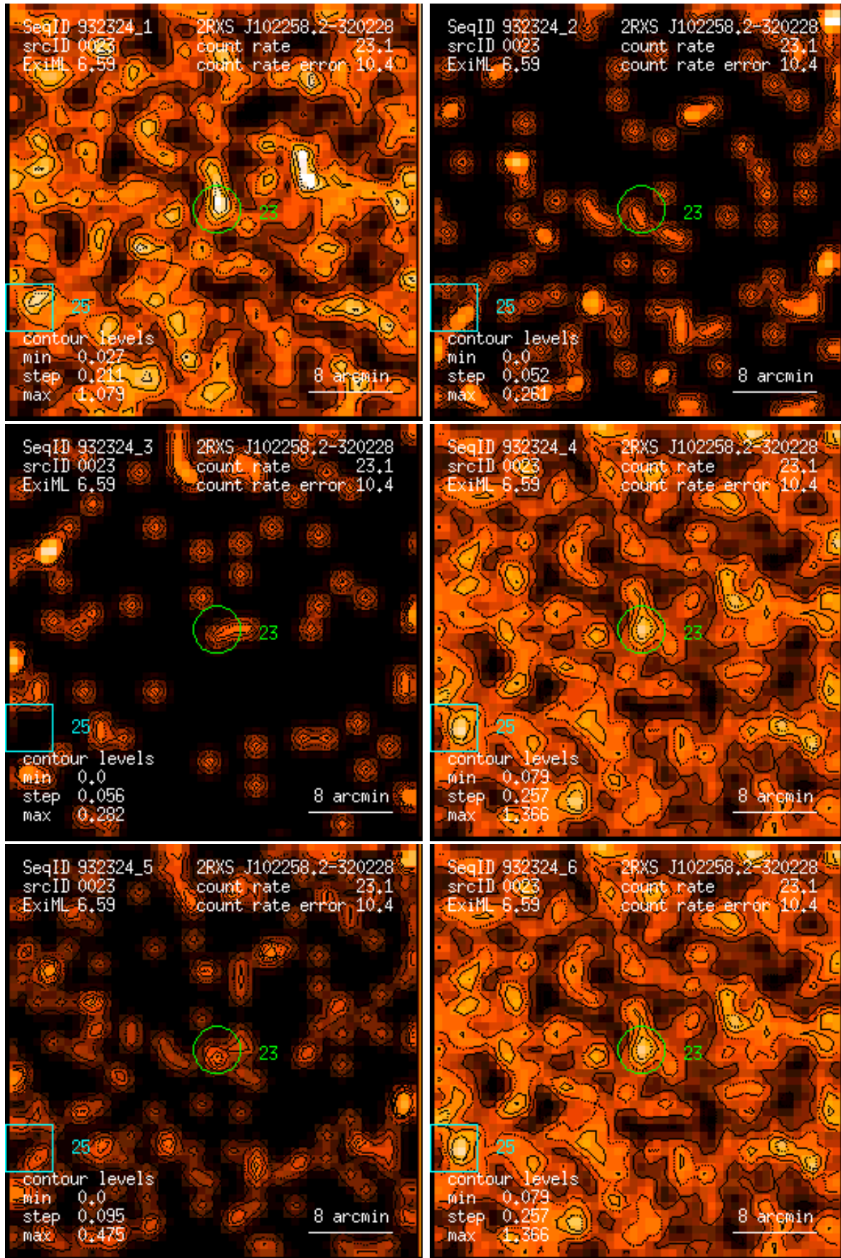
Figure 23: RASS 932324: detection 0023: band rate images, Gaussian filter: (1) PSPC channels 11 – 41, (2) 52 – 90, (3) 91 – 201, (4) 11 – 235, (5) 52 – 201, (6) 11 – 201. Broad band rates in counts/ks. Band rate contour levels in counts/ks/arcmin 2 .
