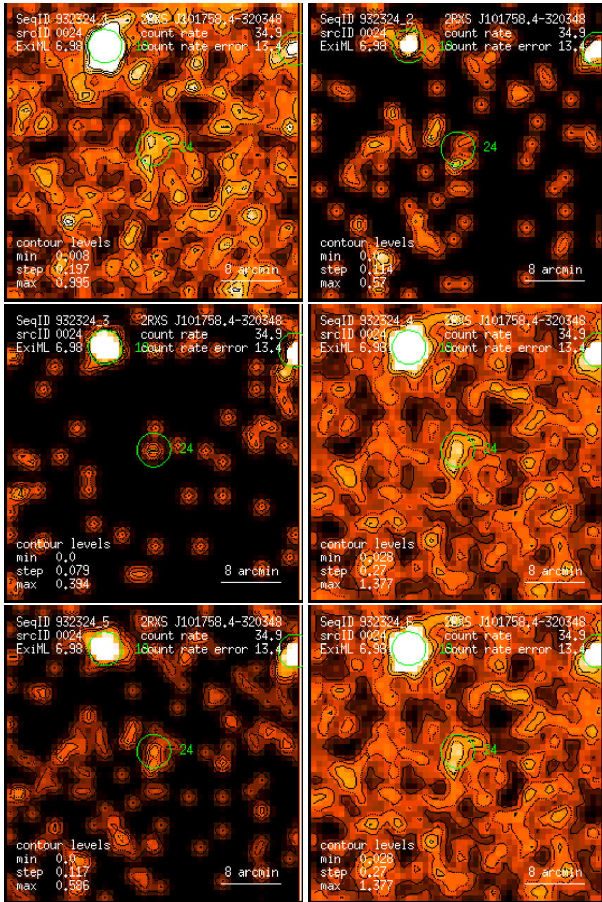
Figure 24: RASS 932324: detection 0024: band rate images, Gaussian filter: (1) PSPC channels 11 – 41, (2) 52 – 90, (3) 91 – 201, (4) 11 – 235, (5) 52 – 201, (6) 11 – 201. Broad band rates in counts/ks. Band rate contour levels in counts/ks/arcmin 2 .
