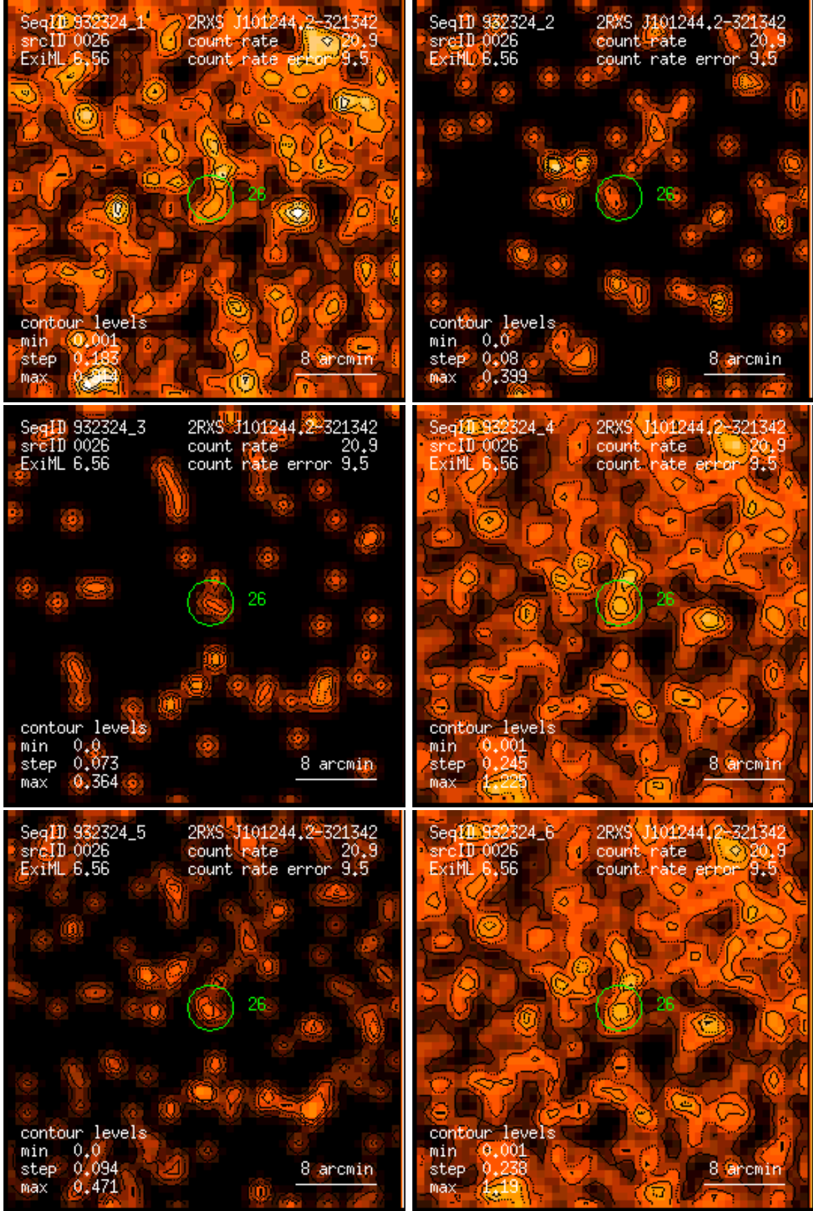
Figure 26: RASS 932324: detection 0026: band rate images, Gaussian filter: (1) PSPC channels 11 – 41, (2) 52 – 90, (3) 91 – 201, (4) 11 – 235, (5) 52 – 201, (6) 11 – 201. Broad band rates in counts/ks. Band rate contour levels in counts/ks/arcmin 2 .
