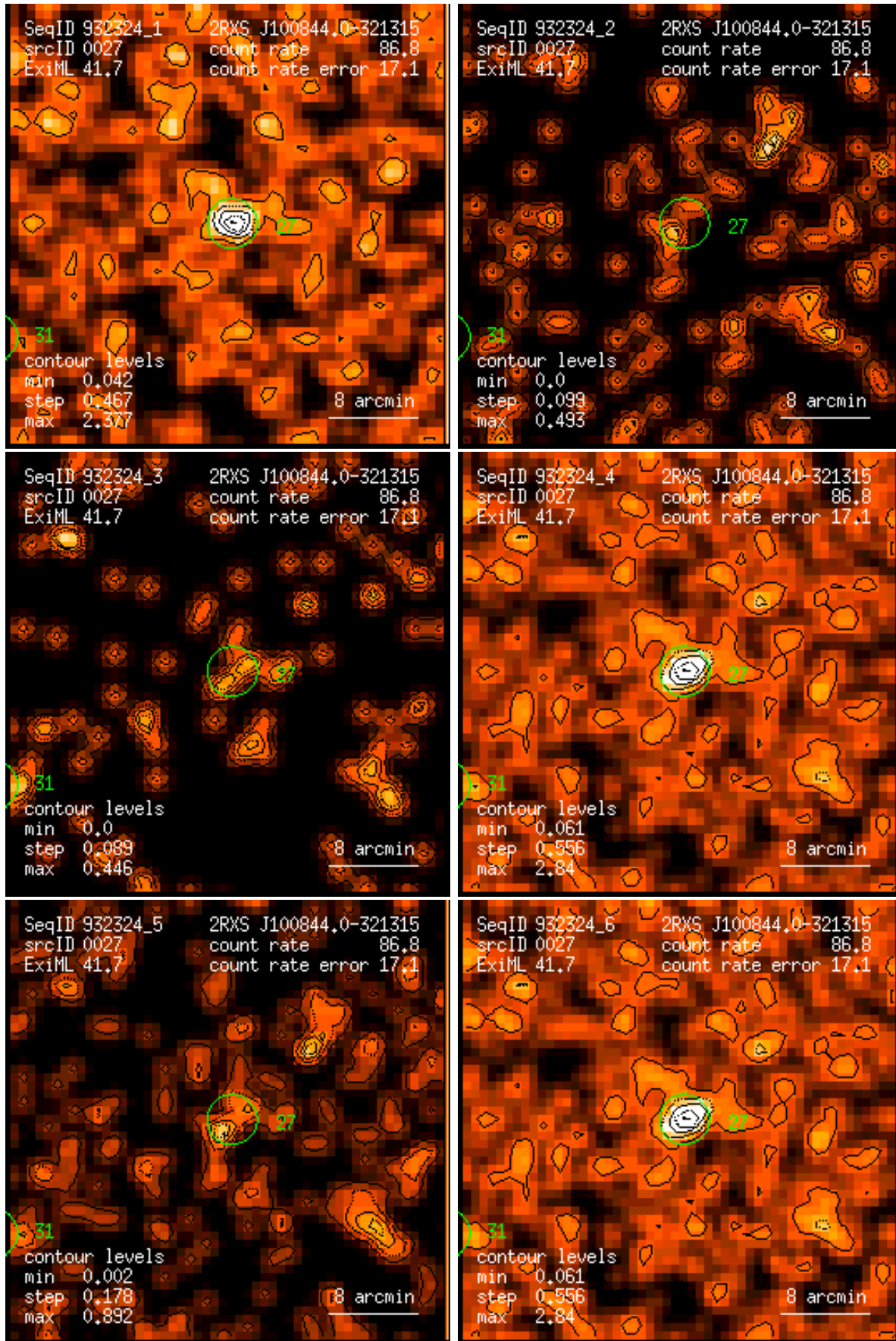
Figure 27: RASS 932324: detection 0027: band rate images, Gaussian filter: (1) PSPC channels 11 – 41, (2) 52 – 90, (3) 91 – 201, (4) 11 – 235, (5) 52 – 201, (6) 11 – 201. Broad band rates in counts/ks. Band rate contour levels in counts/ks/arcmin 2 .
