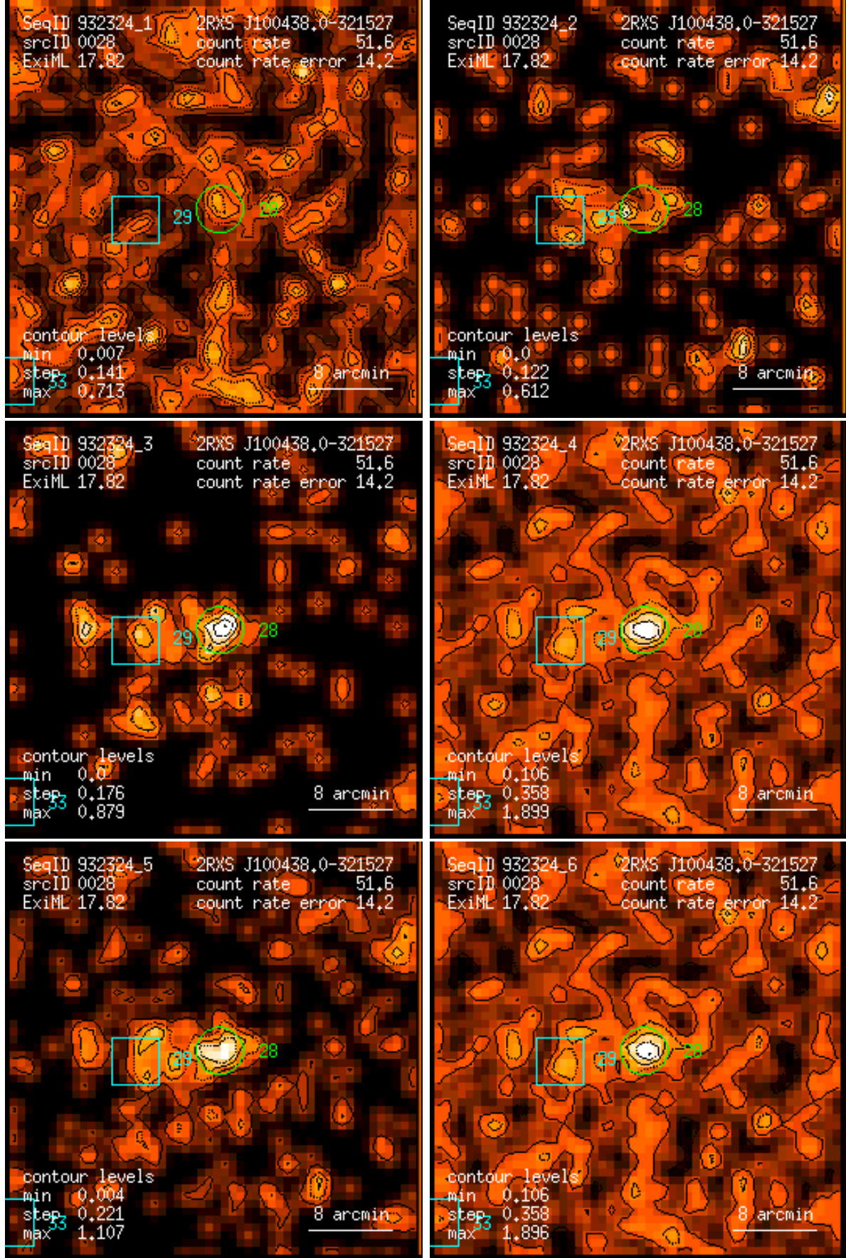
Figure 28: RASS 932324: detection 0028: band rate images, Gaussian filter: (1) PSPC channels 11 – 41, (2) 52 – 90, (3) 91 – 201, (4) 11 – 235, (5) 52 – 201, (6) 11 – 201. Broad band rates in counts/ks. Band rate contour levels in counts/ks/arcmin 2 .
