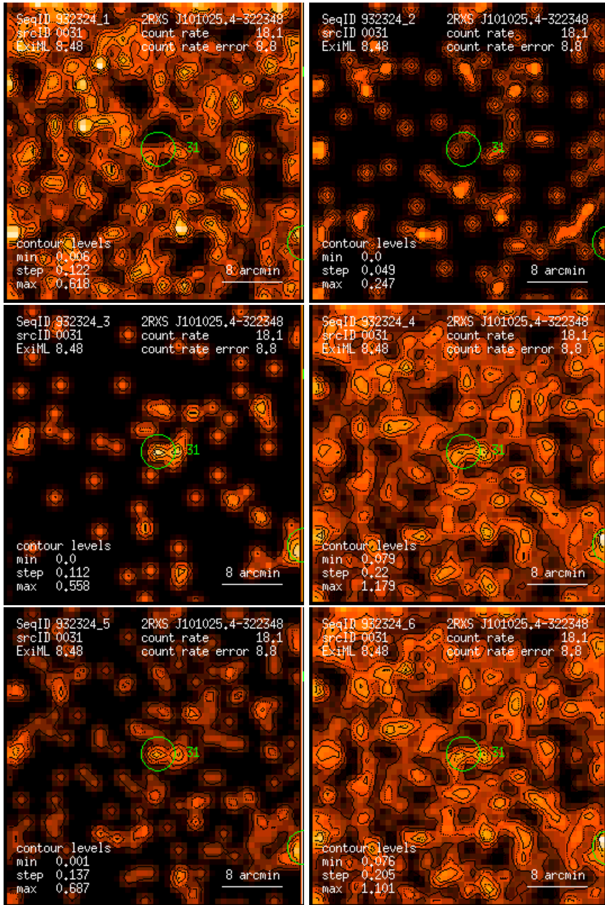
Figure 31: RASS 932324: detection 0031: band rate images, Gaussian filter: (1) PSPC channels 11 – 41, (2) 52 – 90, (3) 91 – 201, (4) 11 – 235, (5) 52 – 201, (6) 11 – 201. Broad band rates in counts/ks. Band rate contour levels in counts/ks/arcmin 2 .
