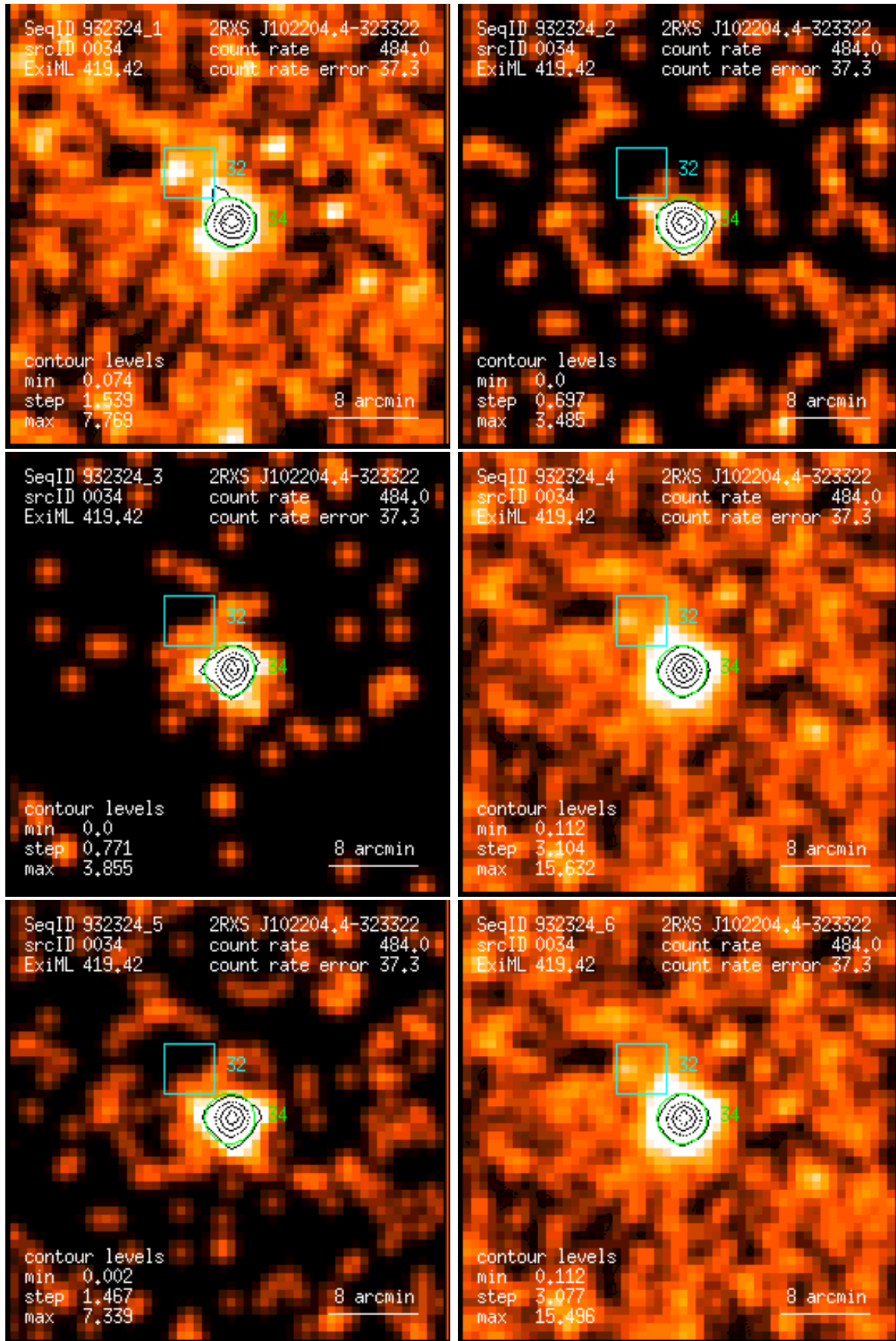
Figure 34: RASS 932324: detection 0034: band rate images, Gaussian filter: (1) PSPC channels 11 – 41, (2) 52 – 90, (3) 91 – 201, (4) 11 – 235, (5) 52 – 201, (6) 11 – 201. Broad band rates in counts/ks. Band rate contour levels in counts/ks/arcmin 2 .
