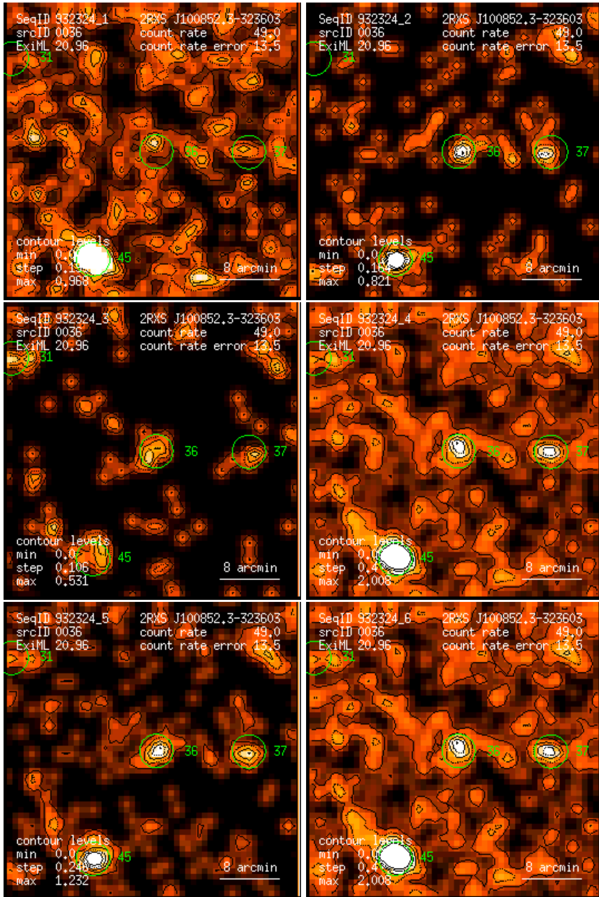
Figure 36: RASS 932324: detection 0036: band rate images, Gaussian filter: (1) PSPC channels 11 – 41, (2) 52 – 90, (3) 91 – 201, (4) 11 – 235, (5) 52 – 201, (6) 11 – 201. Broad band rates in counts/ks. Band rate contour levels in counts/ks/arcmin 2 .
