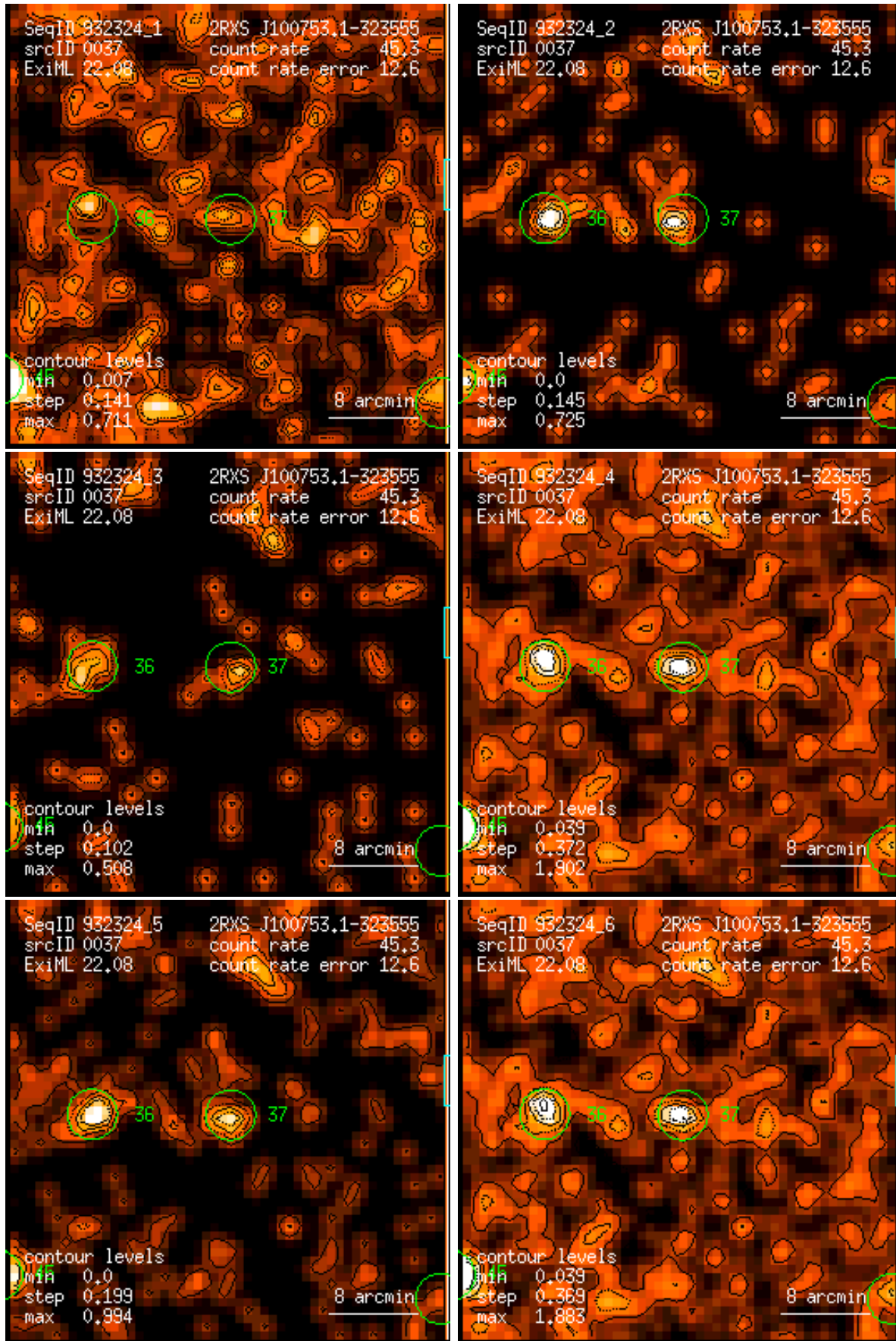
Figure 37: RASS 932324: detection 0037: band rate images, Gaussian filter: (1) PSPC channels 11 – 41, (2) 52 – 90, (3) 91 – 201, (4) 11 – 235, (5) 52 – 201, (6) 11 – 201. Broad band rates in counts/ks. Band rate contour levels in counts/ks/arcmin 2 .
