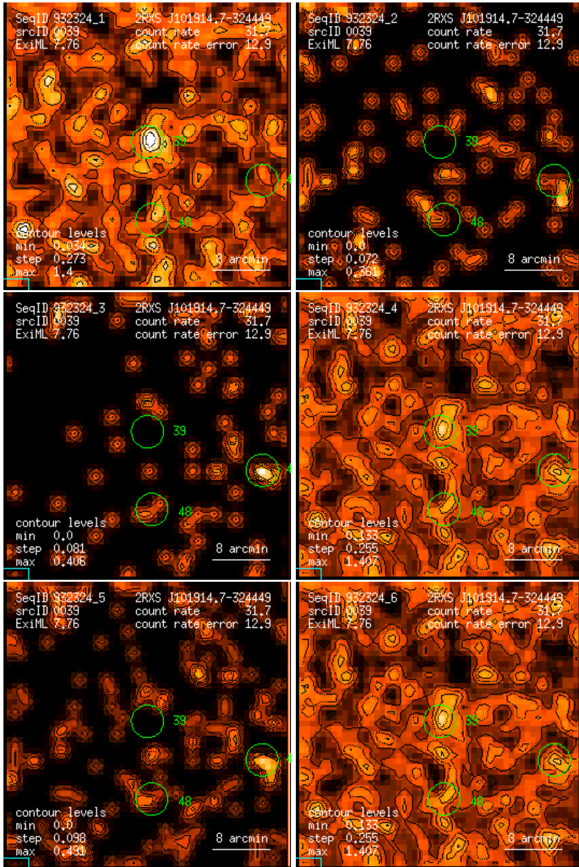
Figure 39: RASS 932324: detection 0039: band rate images, Gaussian filter: (1) PSPC channels 11 – 41, (2) 52 – 90, (3) 91 – 201, (4) 11 – 235, (5) 52 – 201, (6) 11 – 201. Broad band rates in counts/ks. Band rate contour levels in counts/ks/arcmin 2 .
