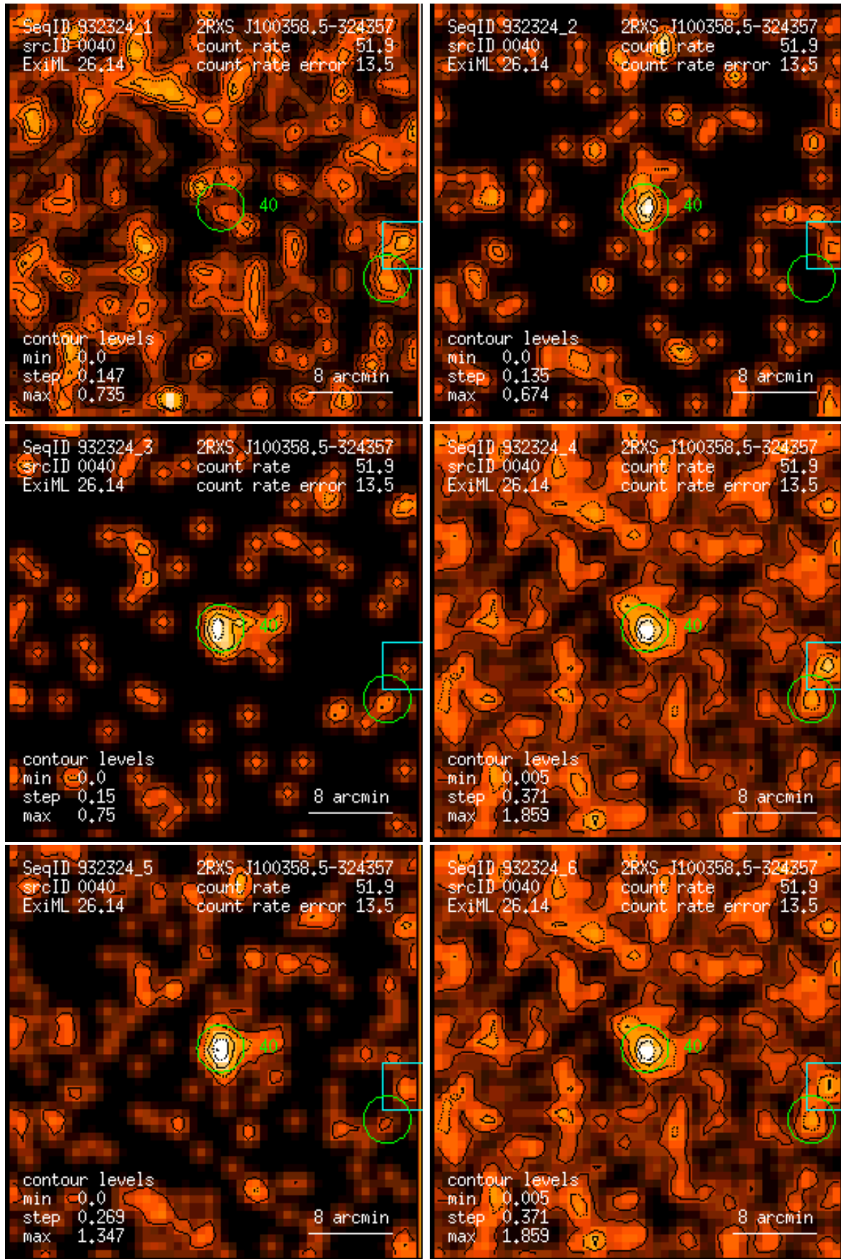
Figure 40: RASS 932324: detection 0040: band rate images, Gaussian filter: (1) PSPC channels 11 – 41, (2) 52 – 90, (3) 91 – 201, (4) 11 – 235, (5) 52 – 201, (6) 11 – 201. Broad band rates in counts/ks. Band rate contour levels in counts/ks/arcmin 2 .
