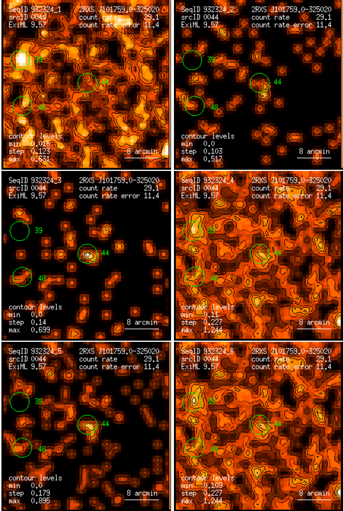
Figure 44: RASS 932324: detection 0044: band rate images, Gaussian filter: (1) PSPC channels 11 – 41, (2) 52 – 90, (3) 91 – 201, (4) 11 – 235, (5) 52 – 201, (6) 11 – 201. Broad band rates in counts/ks. Band rate contour levels in counts/ks/arcmin 2 .
