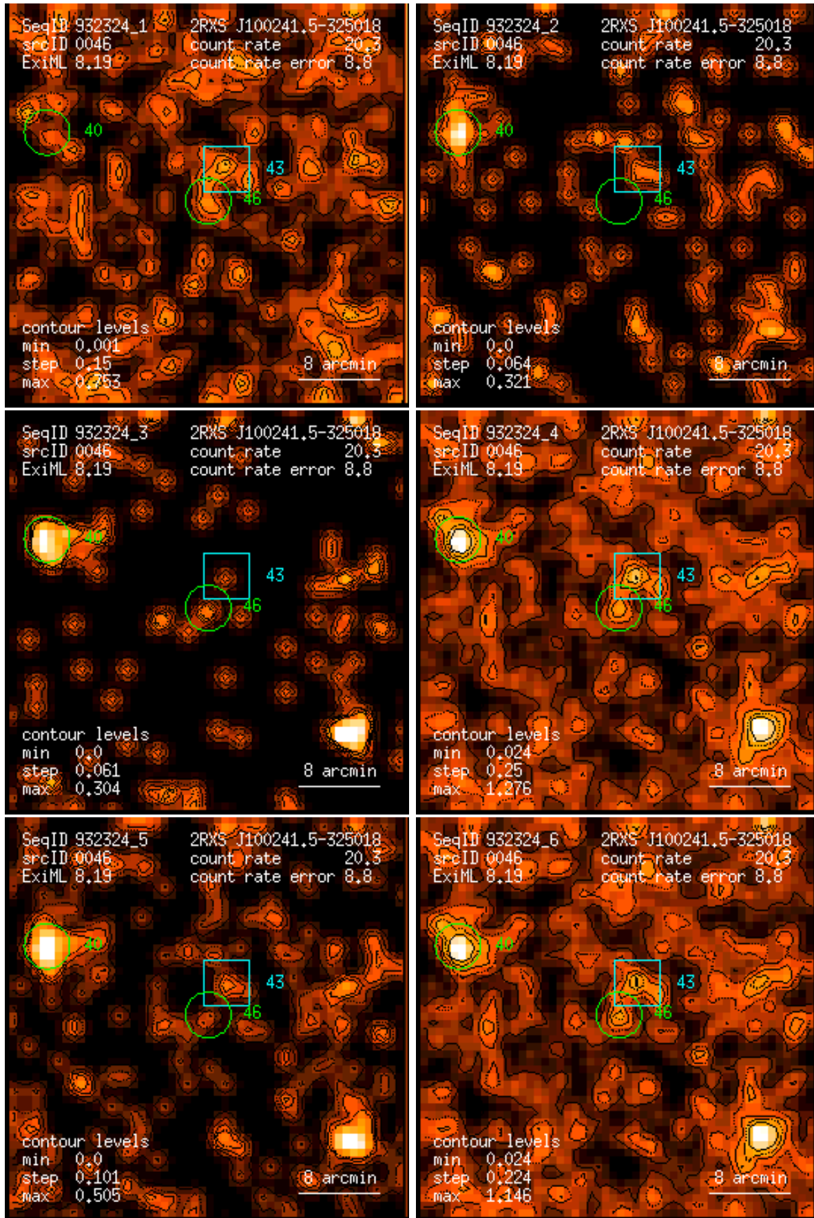
Figure 46: RASS 932324: detection 0046: band rate images, Gaussian filter: (1) PSPC channels 11 – 41, (2) 52 – 90, (3) 91 – 201, (4) 11 – 235, (5) 52 – 201, (6) 11 – 201. Broad band rates in counts/ks. Band rate contour levels in counts/ks/arcmin 2 .
