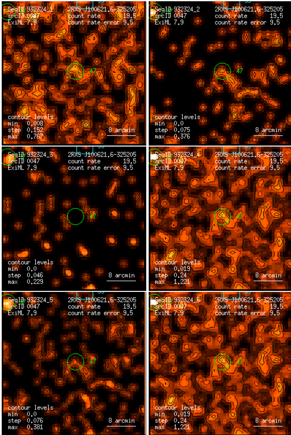
Figure 47: RASS 932324: detection 0047: band rate images, Gaussian filter: (1) PSPC channels 11 – 41, (2) 52 – 90, (3) 91 – 201, (4) 11 – 235, (5) 52 – 201, (6) 11 – 201. Broad band rates in counts/ks. Band rate contour levels in counts/ks/arcmin 2 .
