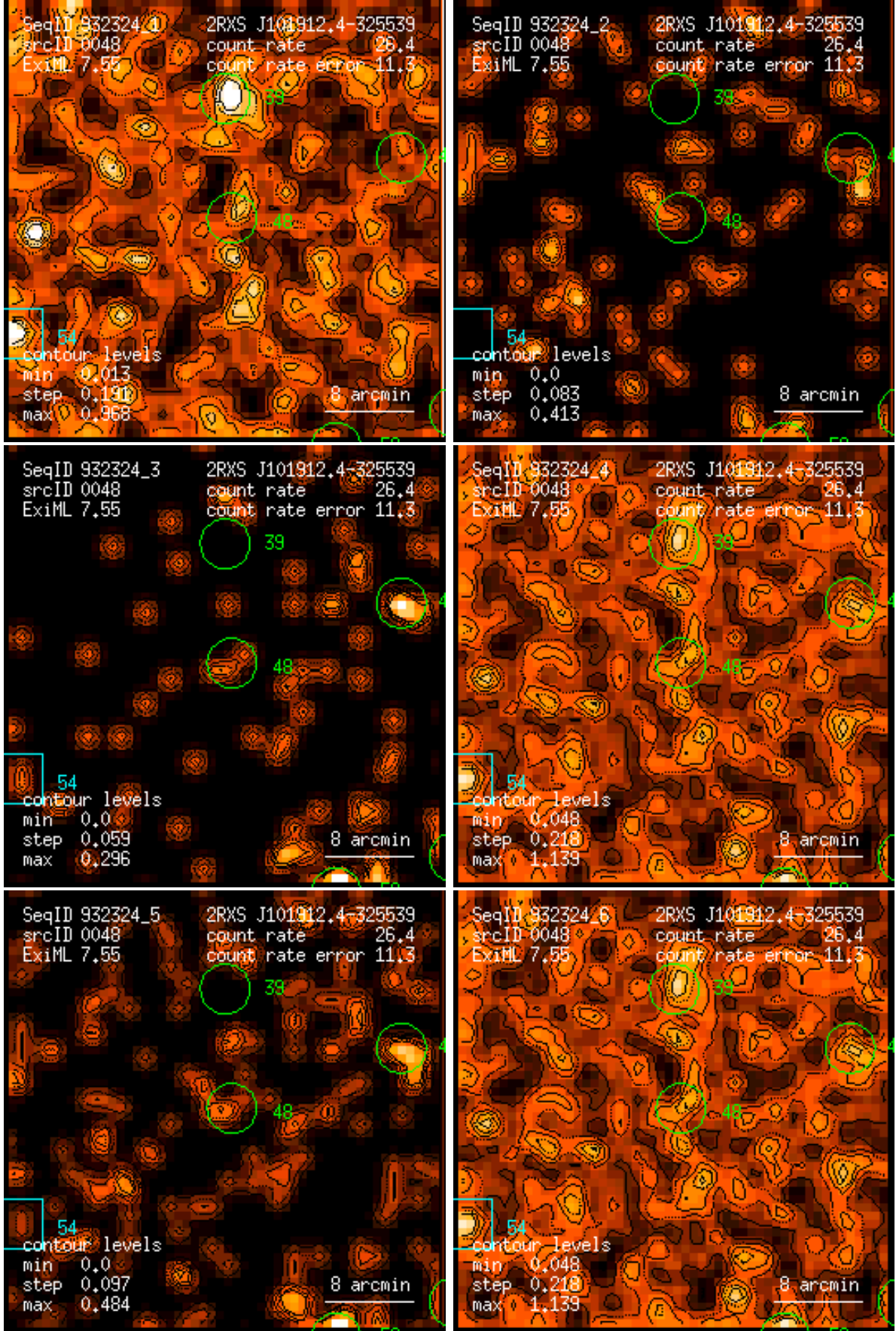
Figure 48: RASS 932324: detection 0048: band rate images, Gaussian filter: (1) PSPC channels 11 – 41, (2) 52 – 90, (3) 91 – 201, (4) 11 – 235, (5) 52 – 201, (6) 11 – 201. Broad band rates in counts/ks. Band rate contour levels in counts/ks/arcmin 2 .
