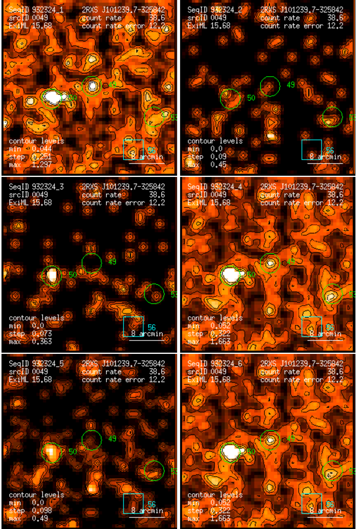
Figure 49: RASS 932324: detection 0049: band rate images, Gaussian filter: (1) PSPC channels 11 – 41, (2) 52 – 90, (3) 91 – 201, (4) 11 – 235, (5) 52 – 201, (6) 11 – 201. Broad band rates in counts/ks. Band rate contour levels in counts/ks/arcmin 2 .
