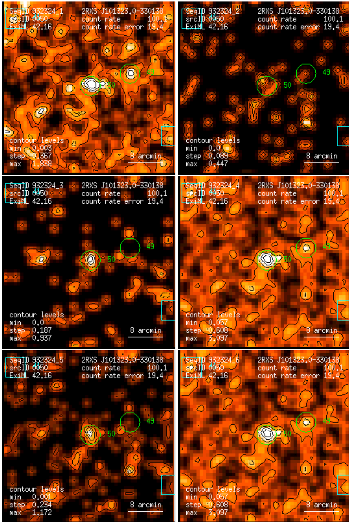
Figure 50: RASS 932324: detection 0050: band rate images, Gaussian filter: (1) PSPC channels 11 – 41, (2) 52 – 90, (3) 91 – 201, (4) 11 – 235, (5) 52 – 201, (6) 11 – 201. Broad band rates in counts/ks. Band rate contour levels in counts/ks/arcmin 2 .
