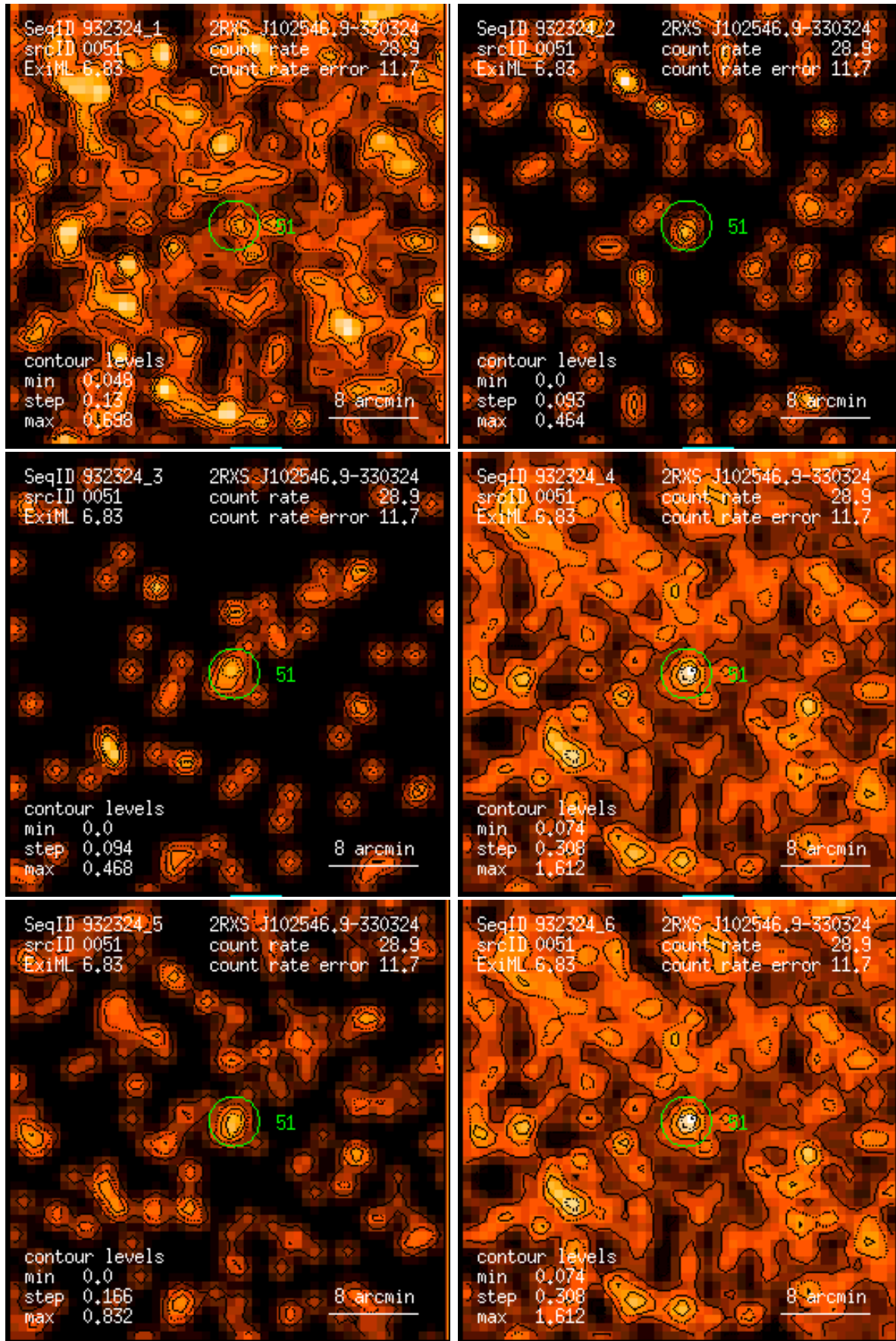
Figure 51: RASS 932324: detection 0051: band rate images, Gaussian filter: (1) PSPC channels 11 – 41, (2) 52 – 90, (3) 91 – 201, (4) 11 – 235, (5) 52 – 201, (6) 11 – 201. Broad band rates in counts/ks. Band rate contour levels in counts/ks/arcmin 2 .
