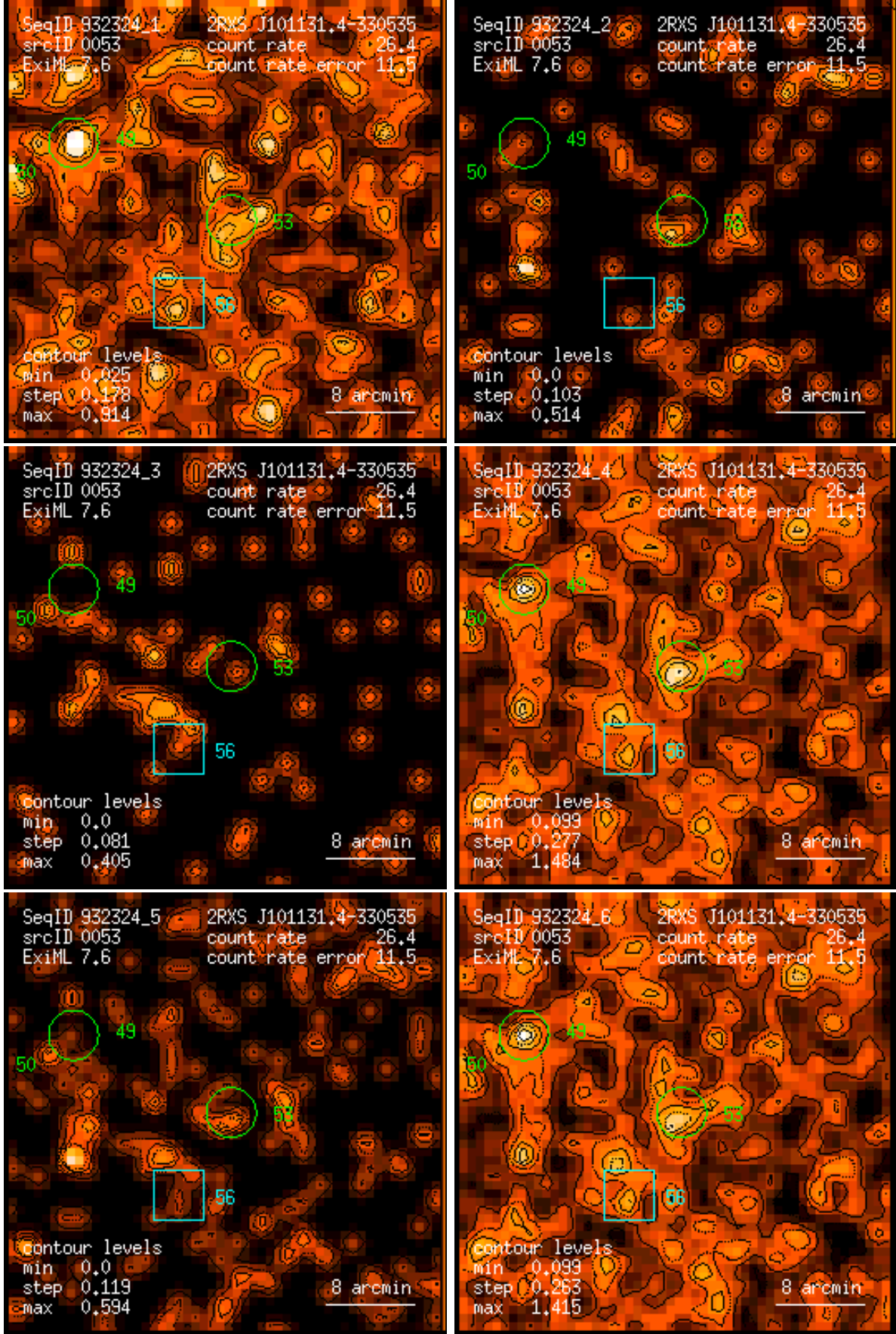
Figure 53: RASS 932324: detection 0053: band rate images, Gaussian filter: (1) PSPC channels 11 – 41, (2) 52 – 90, (3) 91 – 201, (4) 11 – 235, (5) 52 – 201, (6) 11 – 201. Broad band rates in counts/ks. Band rate contour levels in counts/ks/arcmin 2 .
