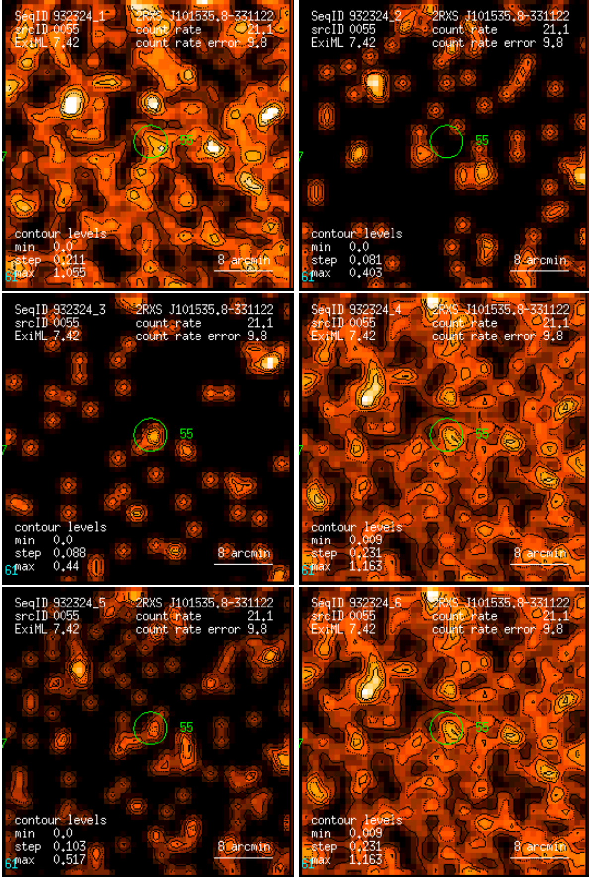
Figure 55: RASS 932324: detection 0055: band rate images, Gaussian filter: (1) PSPC channels 11 – 41, (2) 52 – 90, (3) 91 – 201, (4) 11 – 235, (5) 52 – 201, (6) 11 – 201. Broad band rates in counts/ks. Band rate contour levels in counts/ks/arcmin 2 .
