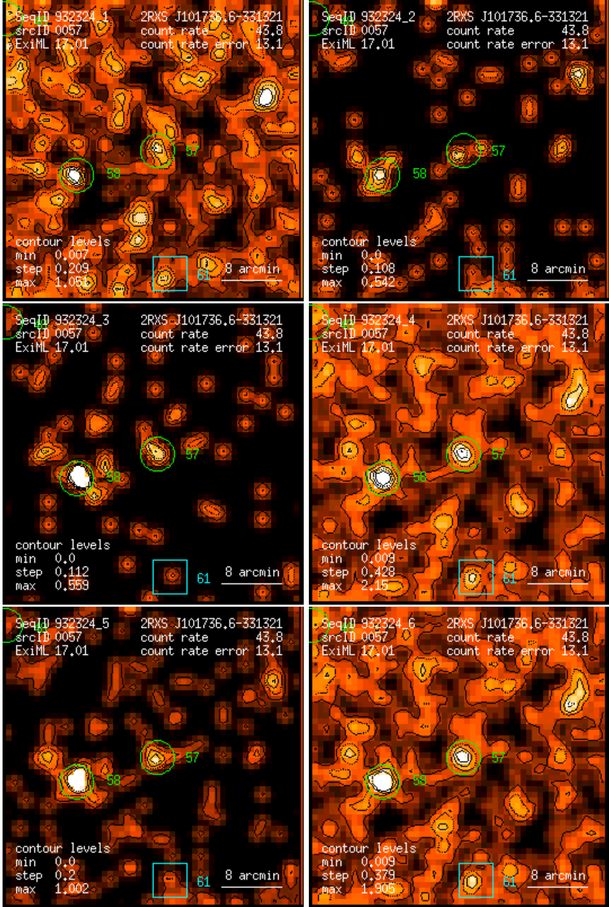
Figure 57: RASS 932324: detection 0057: band rate images, Gaussian filter: (1) PSPC channels 11 – 41, (2) 52 – 90, (3) 91 – 201, (4) 11 – 235, (5) 52 – 201, (6) 11 – 201. Broad band rates in counts/ks. Band rate contour levels in counts/ks/arcmin 2 .
