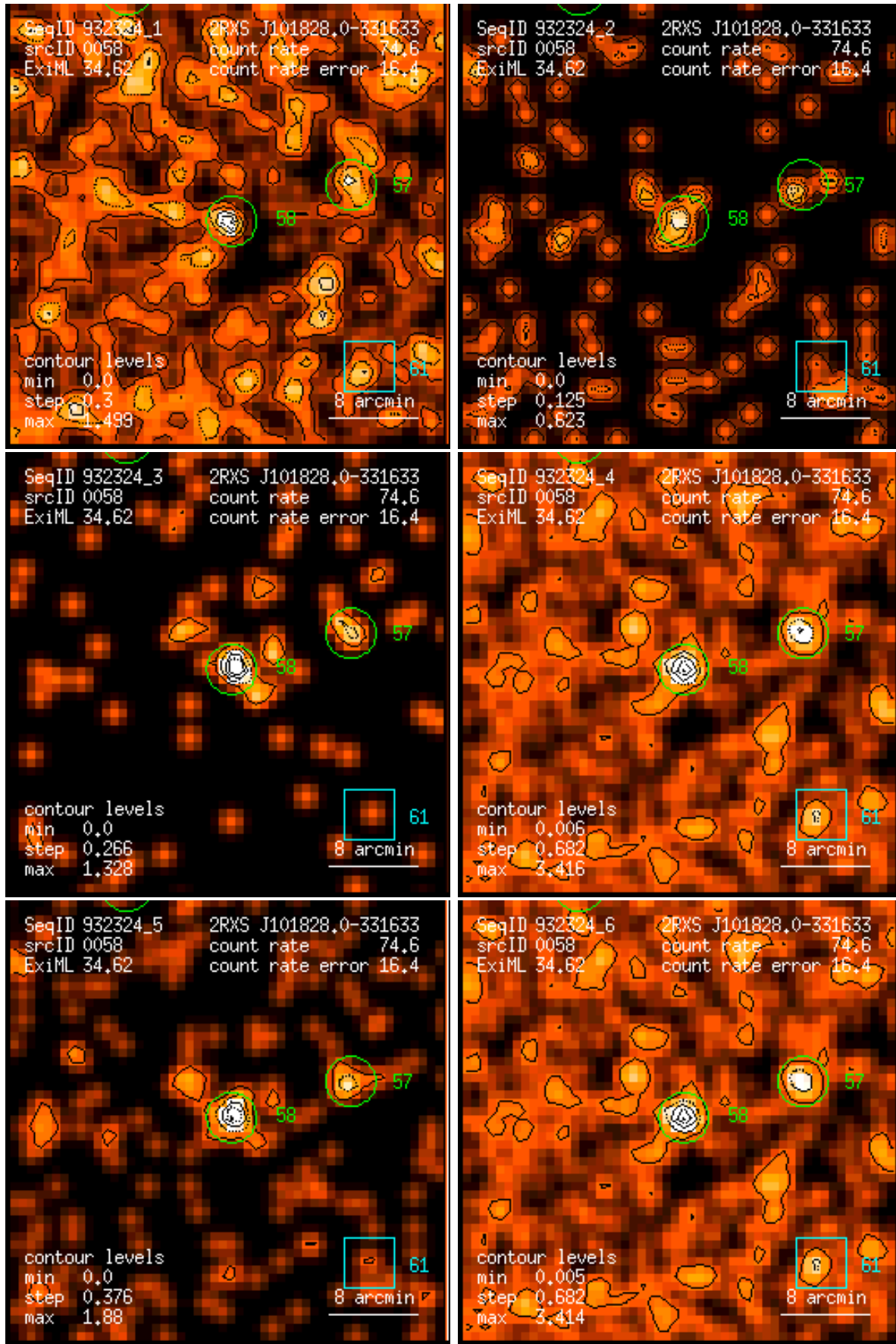
Figure 58: RASS 932324: detection 0058: band rate images, Gaussian filter: (1) PSPC channels 11 – 41, (2) 52 – 90, (3) 91 – 201, (4) 11 – 235, (5) 52 – 201, (6) 11 – 201. Broad band rates in counts/ks. Band rate contour levels in counts/ks/arcmin 2 .
