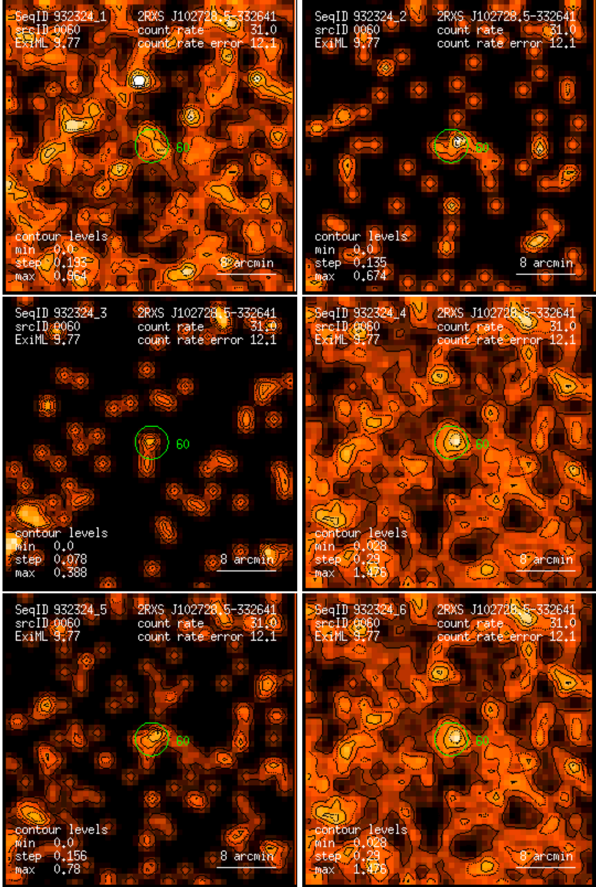
Figure 60: RASS 932324: detection 0060: band rate images, Gaussian filter: (1) PSPC channels 11 – 41, (2) 52 – 90, (3) 91 – 201, (4) 11 – 235, (5) 52 – 201, (6) 11 – 201. Broad band rates in counts/ks. Band rate contour levels in counts/ks/arcmin 2 .
