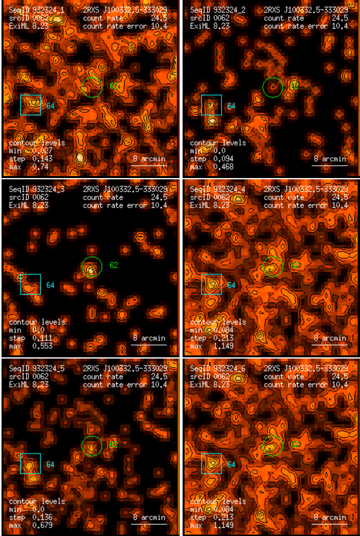
Figure 62: RASS 932324: detection 0062: band rate images, Gaussian filter: (1) PSPC channels 11 – 41, (2) 52 – 90, (3) 91 – 201, (4) 11 – 235, (5) 52 – 201, (6) 11 – 201. Broad band rates in counts/ks. Band rate contour levels in counts/ks/arcmin 2 .
