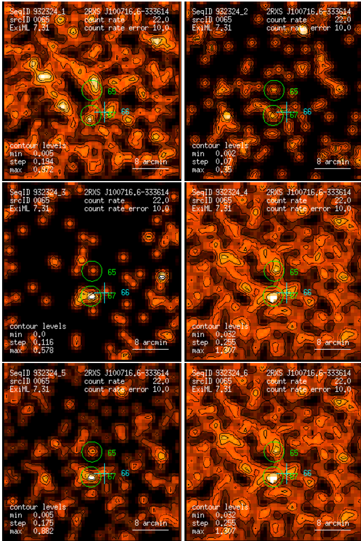
Figure 65: RASS 932324: detection 0065: band rate images, Gaussian filter: (1) PSPC channels 11 – 41, (2) 52 – 90, (3) 91 – 201, (4) 11 – 235, (5) 52 – 201, (6) 11 – 201. Broad band rates in counts/ks. Band rate contour levels in counts/ks/arcmin 2 .
