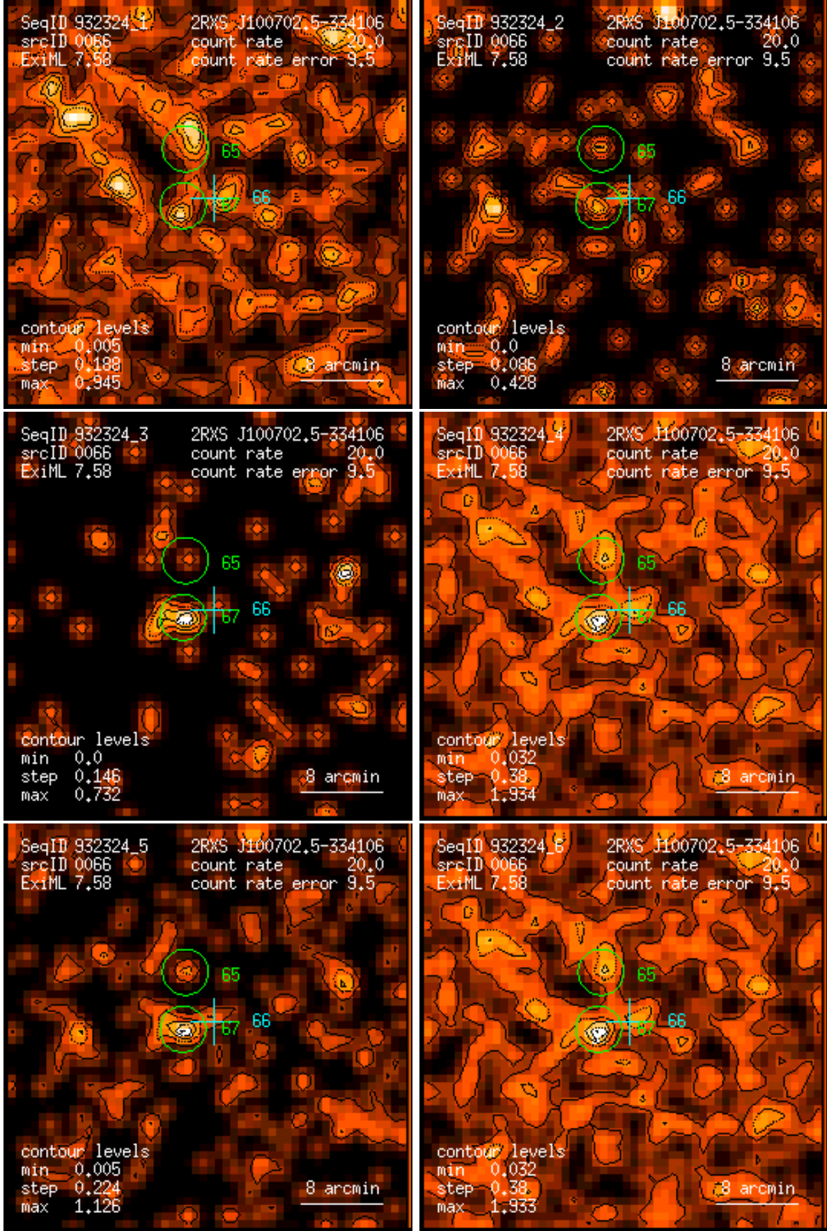
Figure 66: RASS 932324: detection 0066: band rate images, Gaussian filter: (1) PSPC channels 11 – 41, (2) 52 – 90, (3) 91 – 201, (4) 11 – 235, (5) 52 – 201, (6) 11 – 201. Broad band rates in counts/ks. Band rate contour levels in counts/ks/arcmin 2 .
